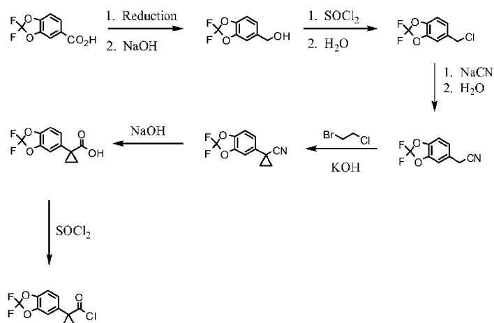
Scheme 1. Synthesis of the acid chloride moiety.
