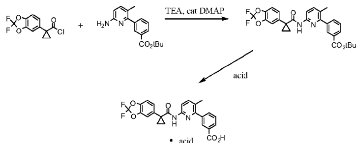
Scheme 3. Formation of an acid salt of 3-(6-(1-(2,2-difluorobenzo[d][1,3]dioxol-5-yl) cyclopropanecarboxamido)-3-methylpyridin-2-yl)benzoic acid.
