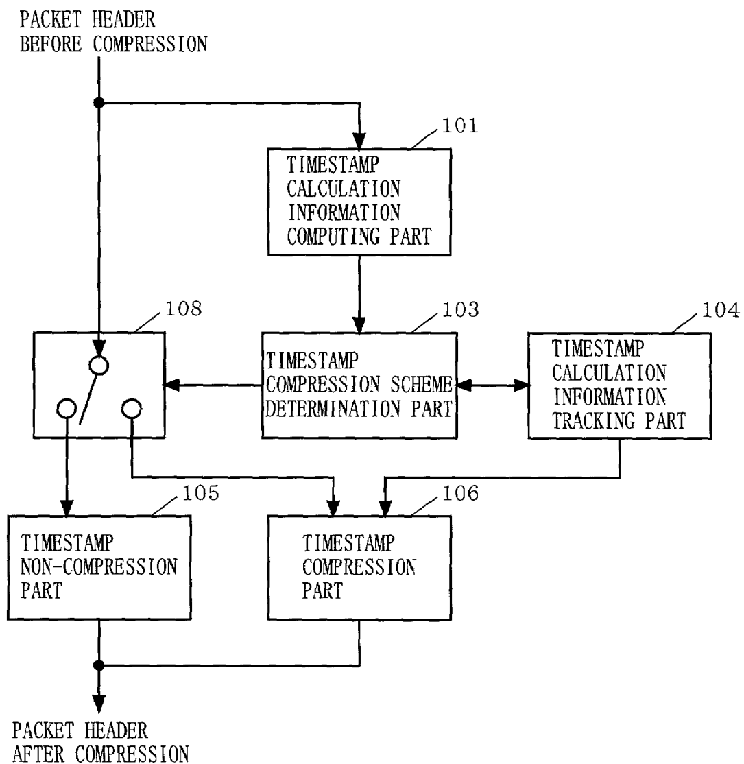
FIG. 15 PRIOR ART
