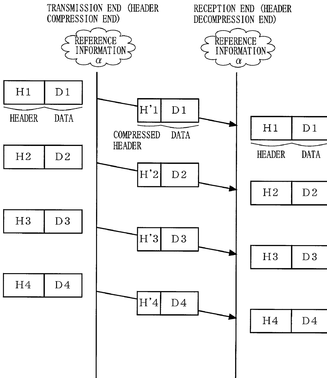
FIG. 10 PRIOR ART
