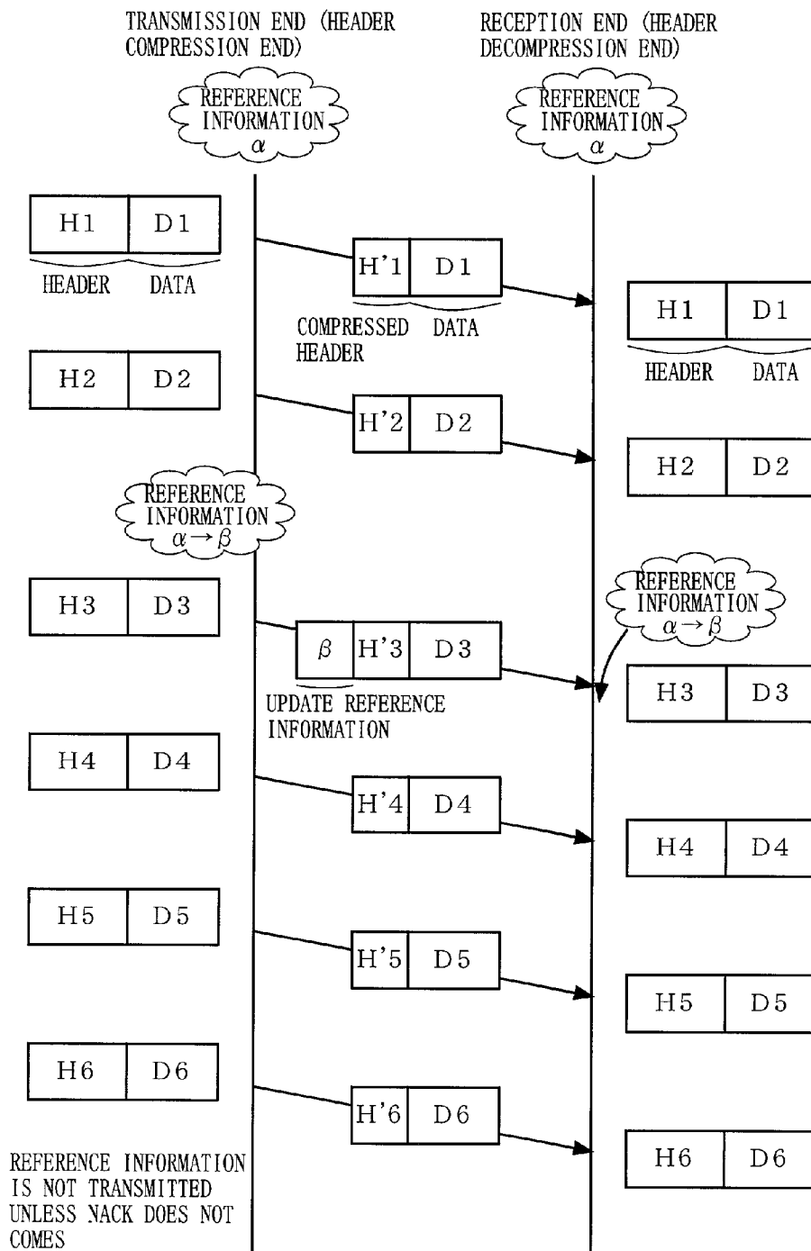
FIG. 11 PRIOR ART
