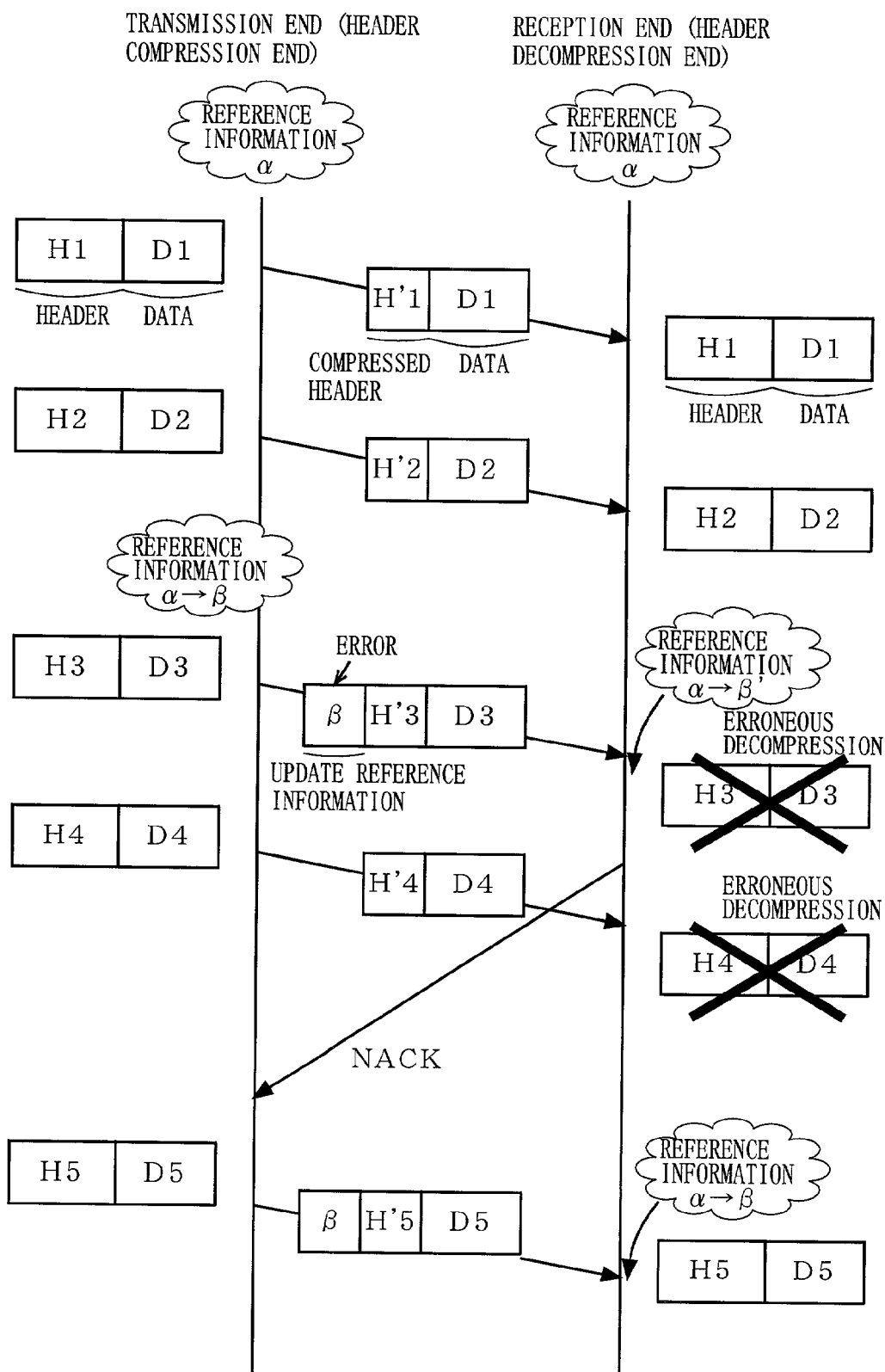
FIG. 12 PRIOR ART
