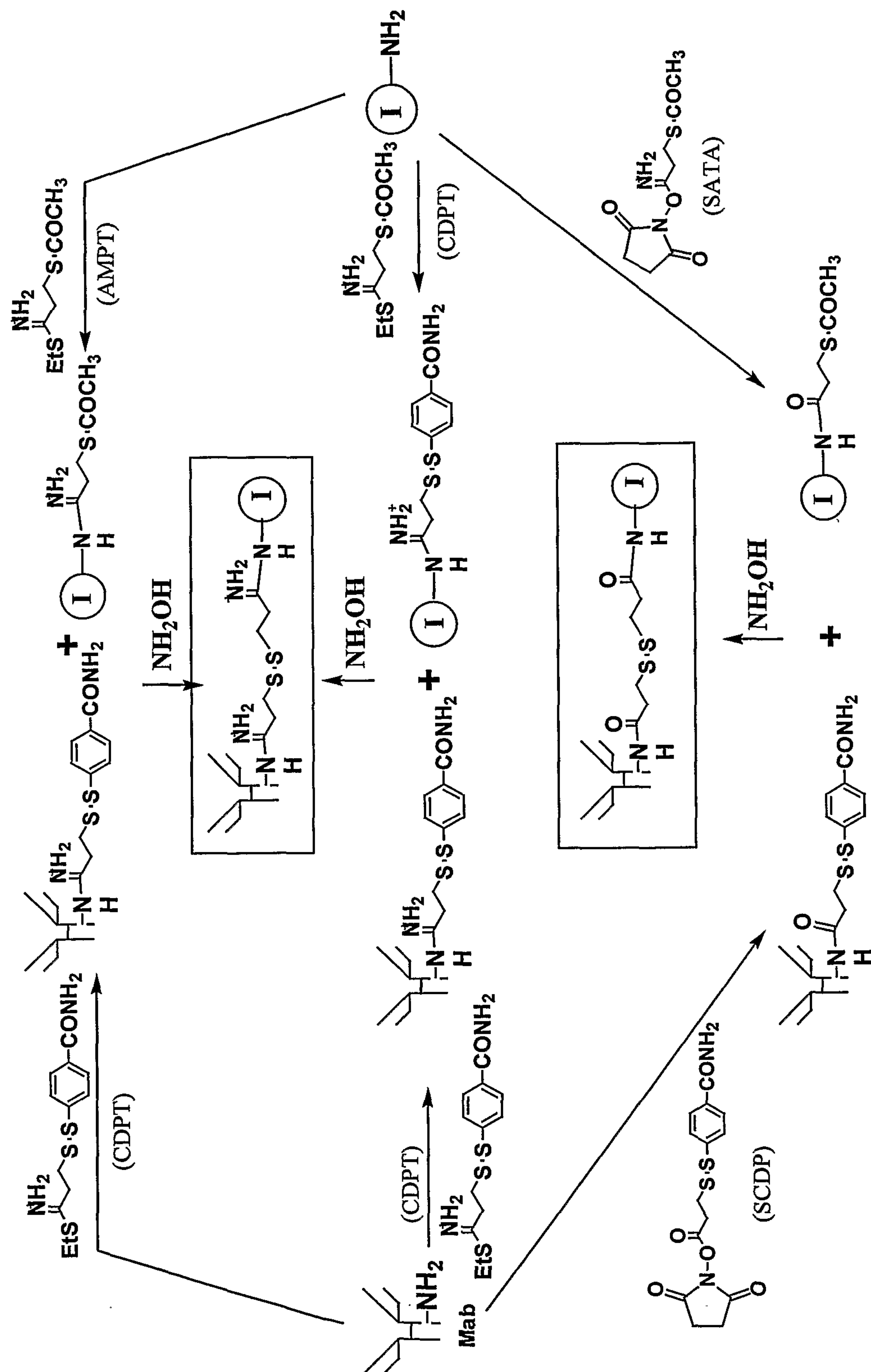
Scheme 11.
