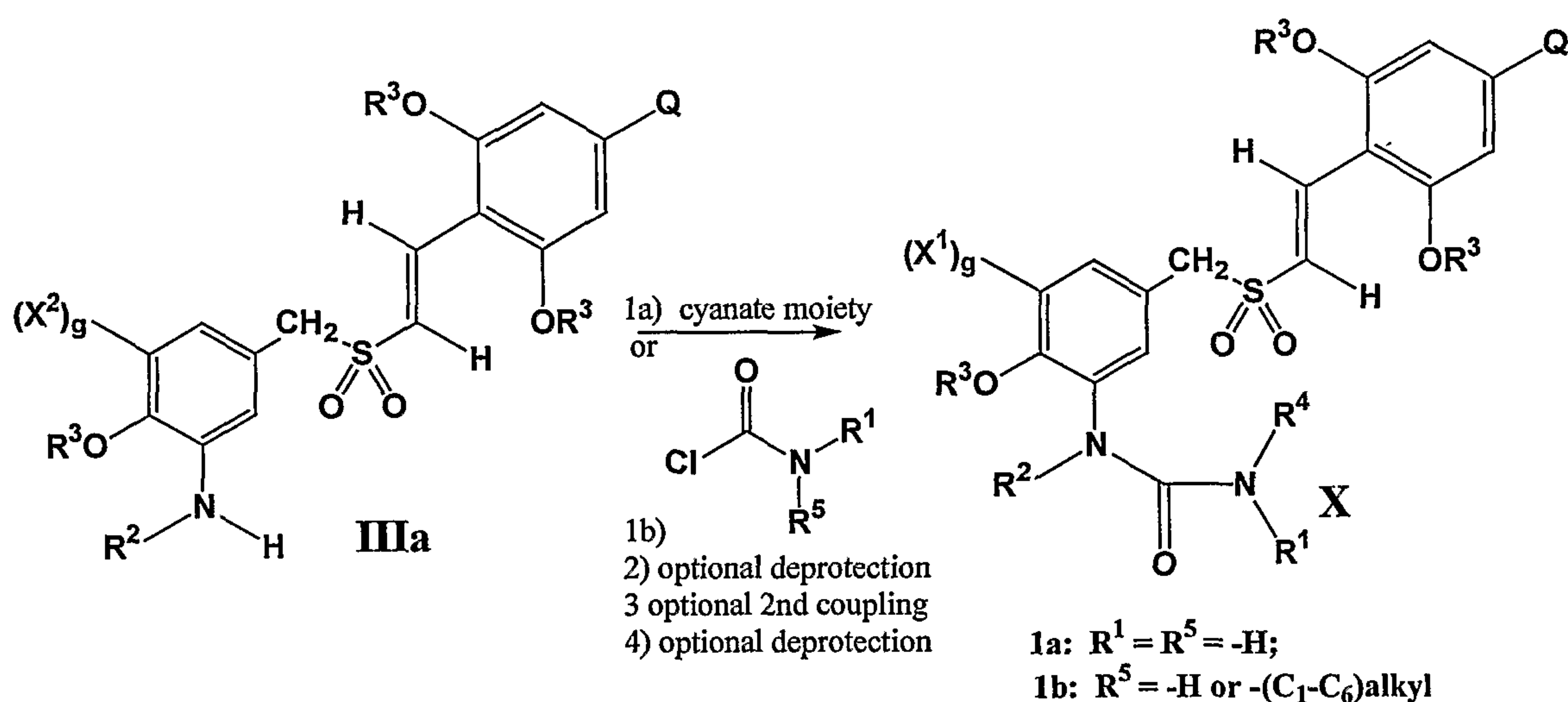
Scheme 8:
