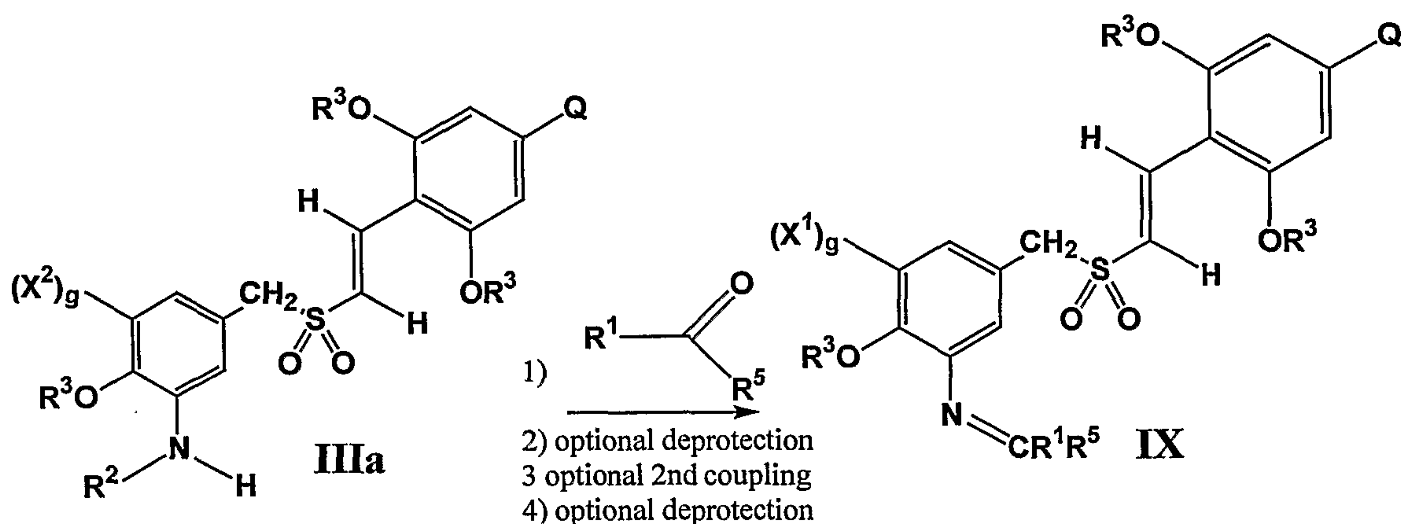
Scheme 7:
