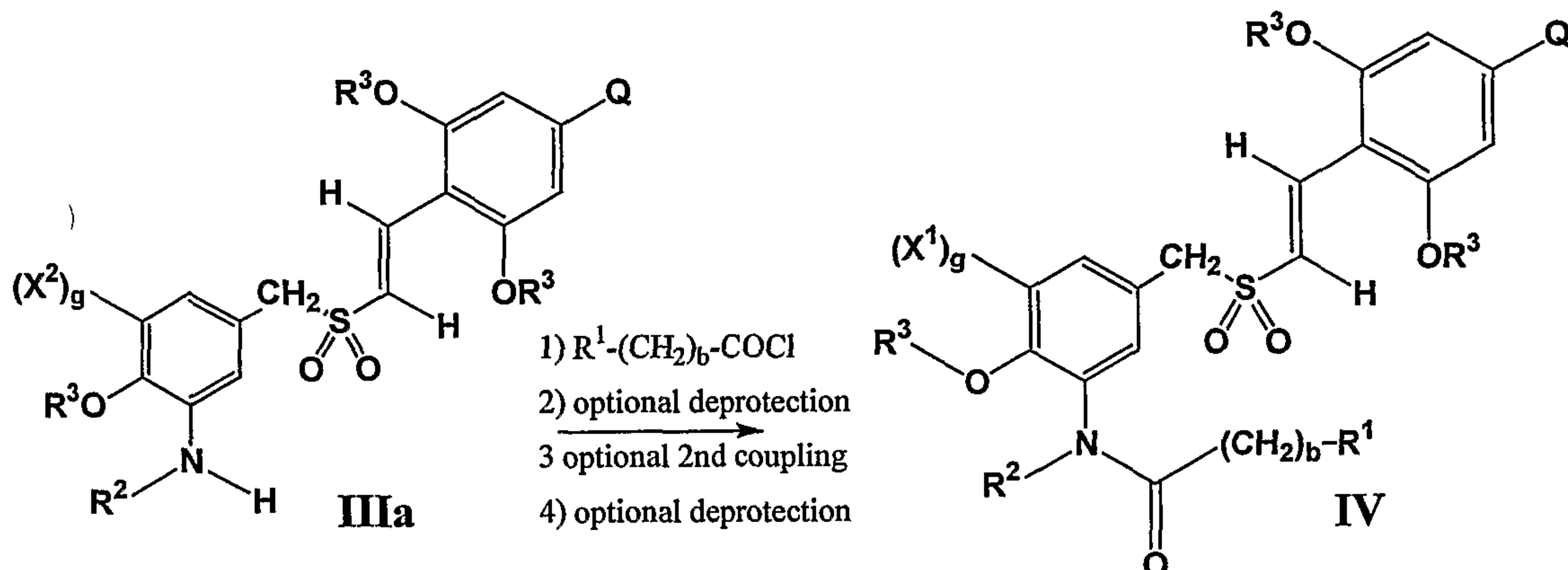
Scheme 2:
