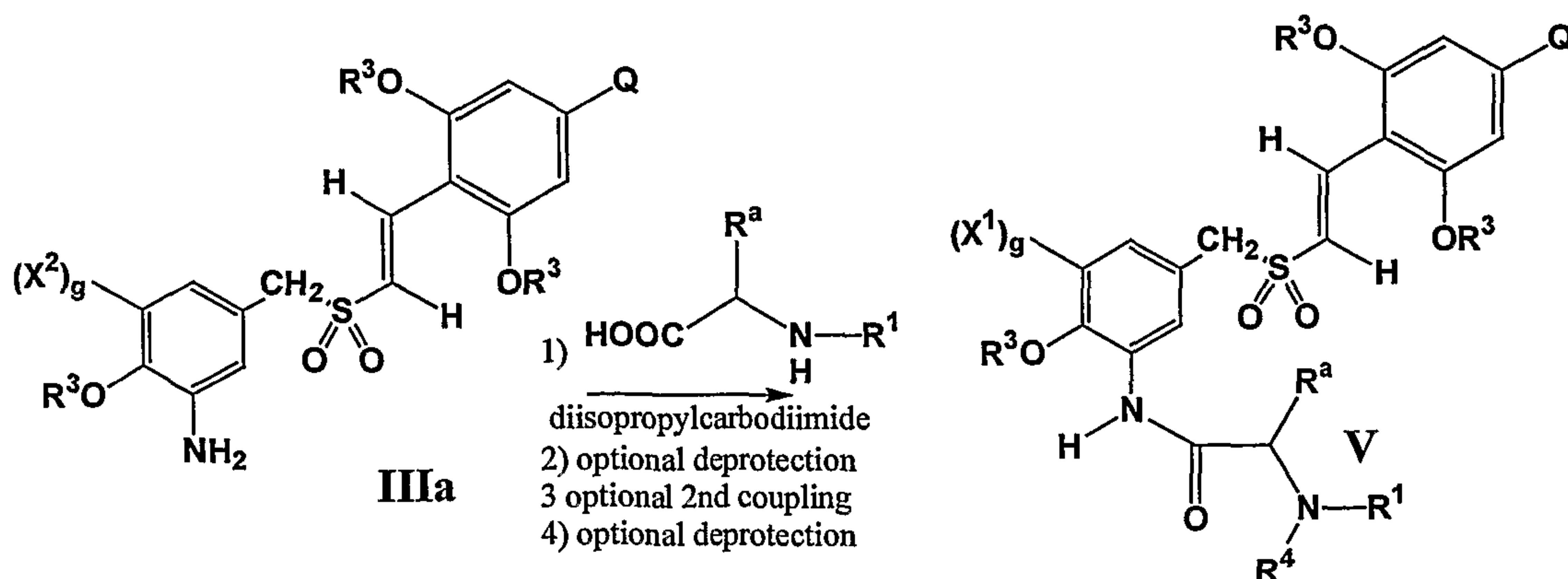
Scheme 3:
