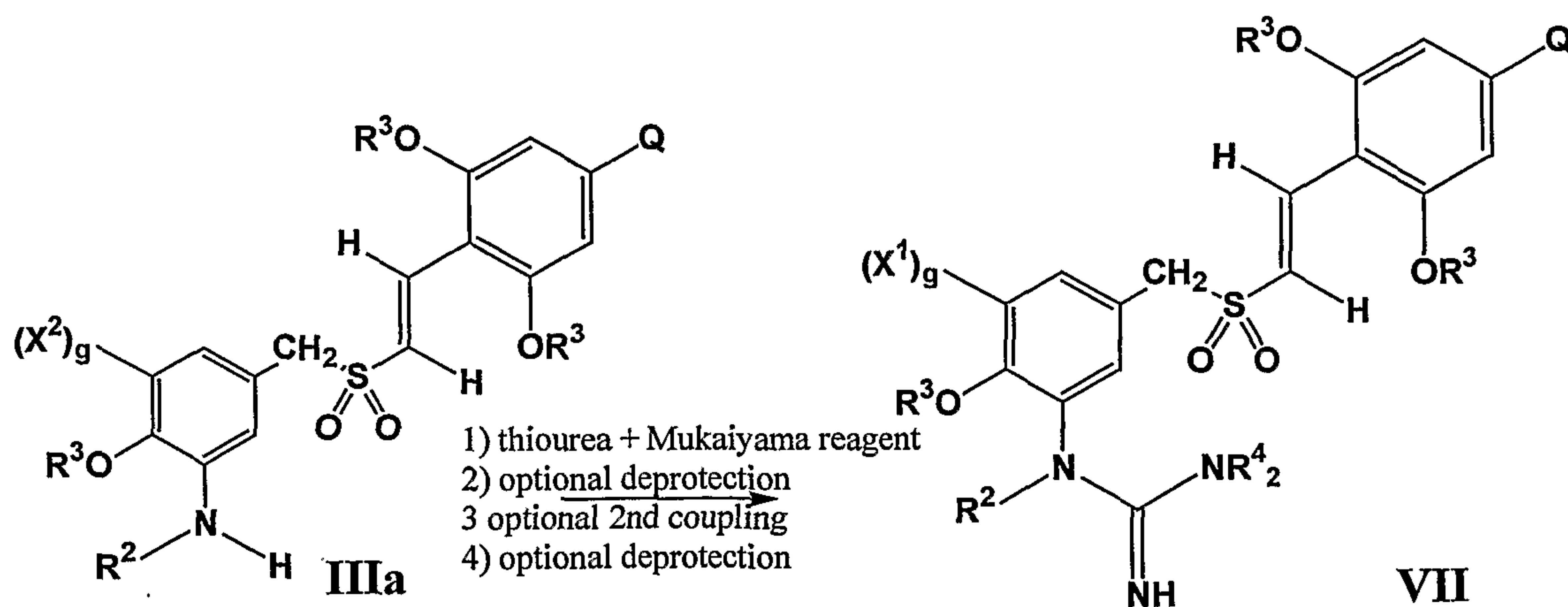
Scheme 5:
