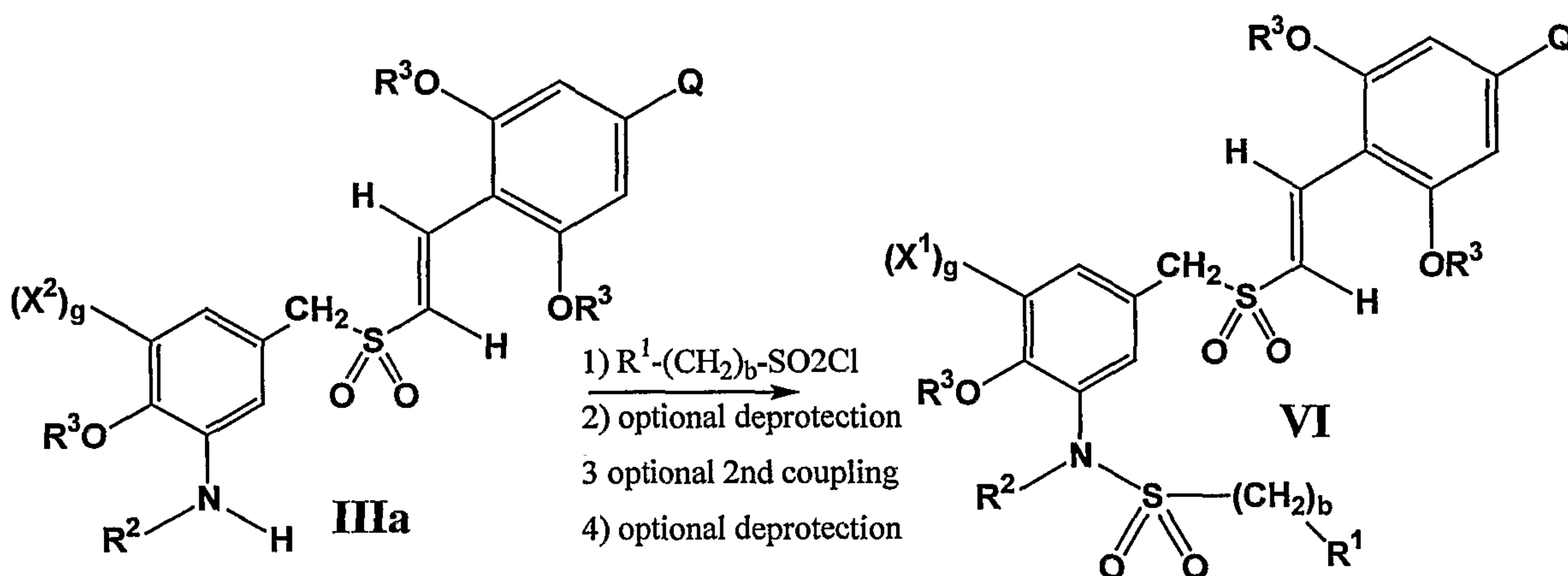
5 Scheme 4:
