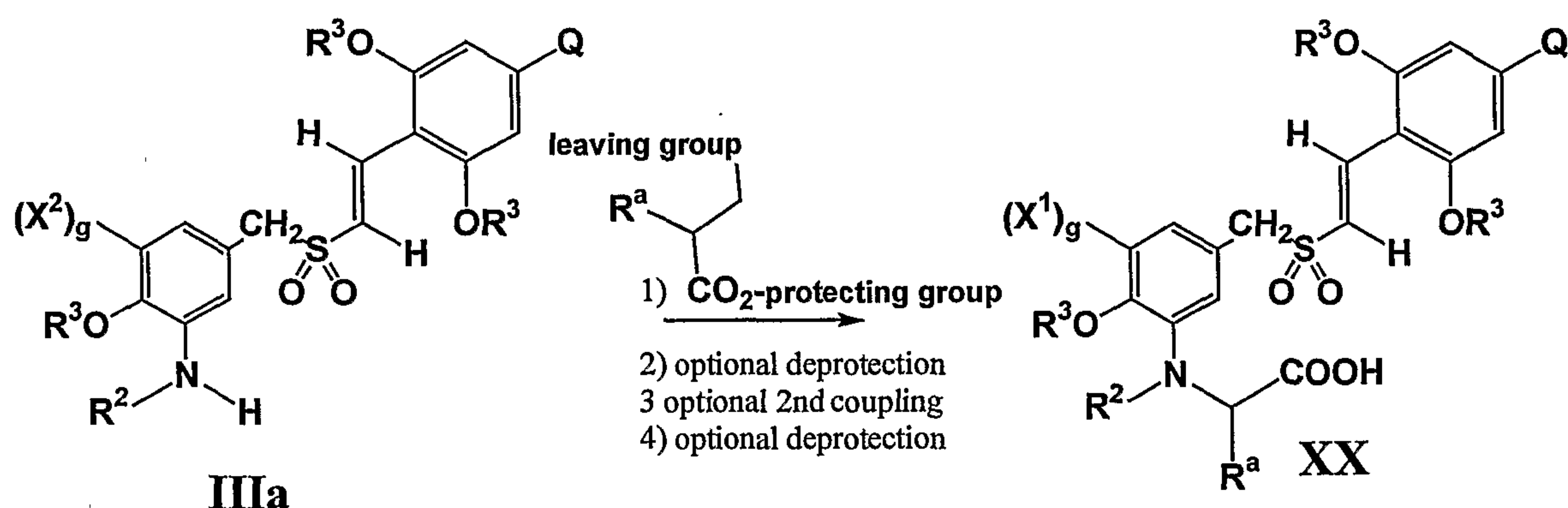
Scheme 9:
