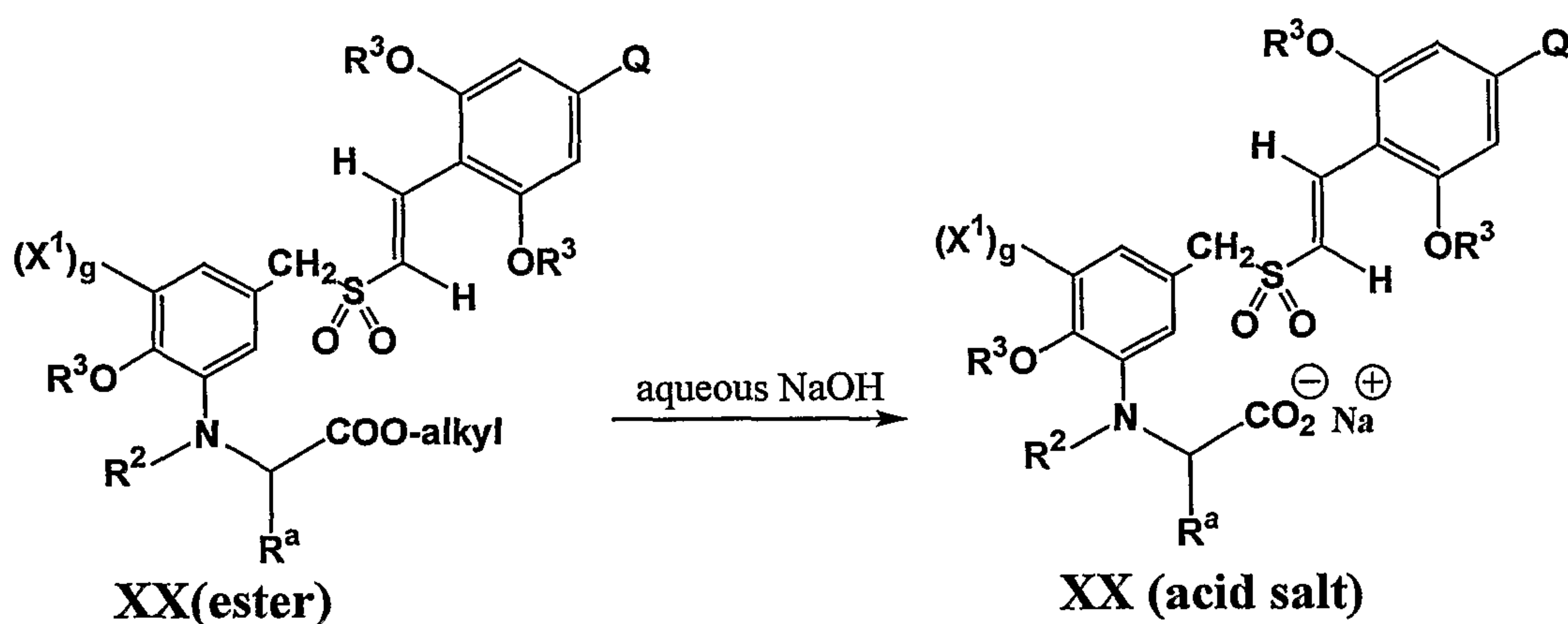
Scheme 10:
