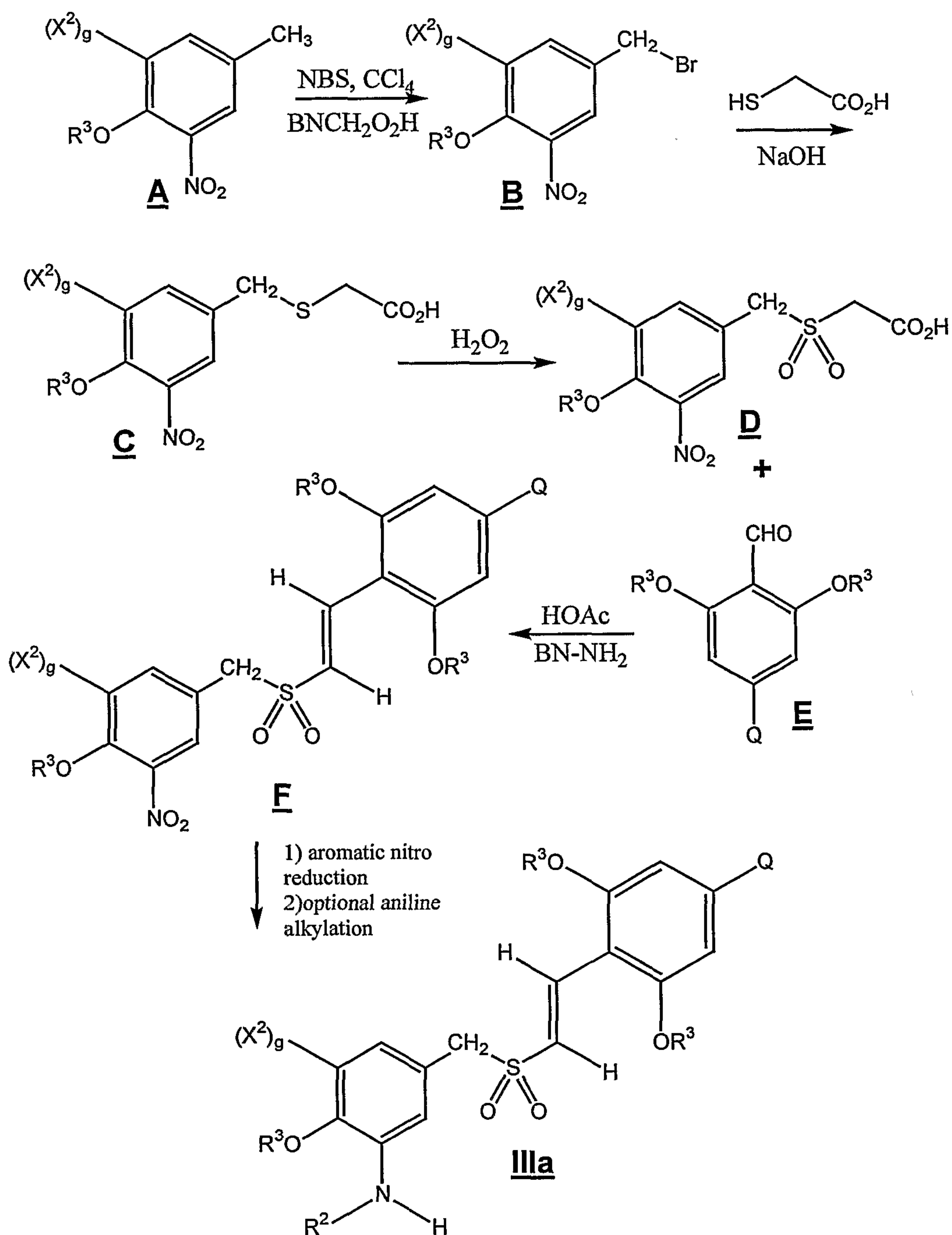
Scheme 1:
