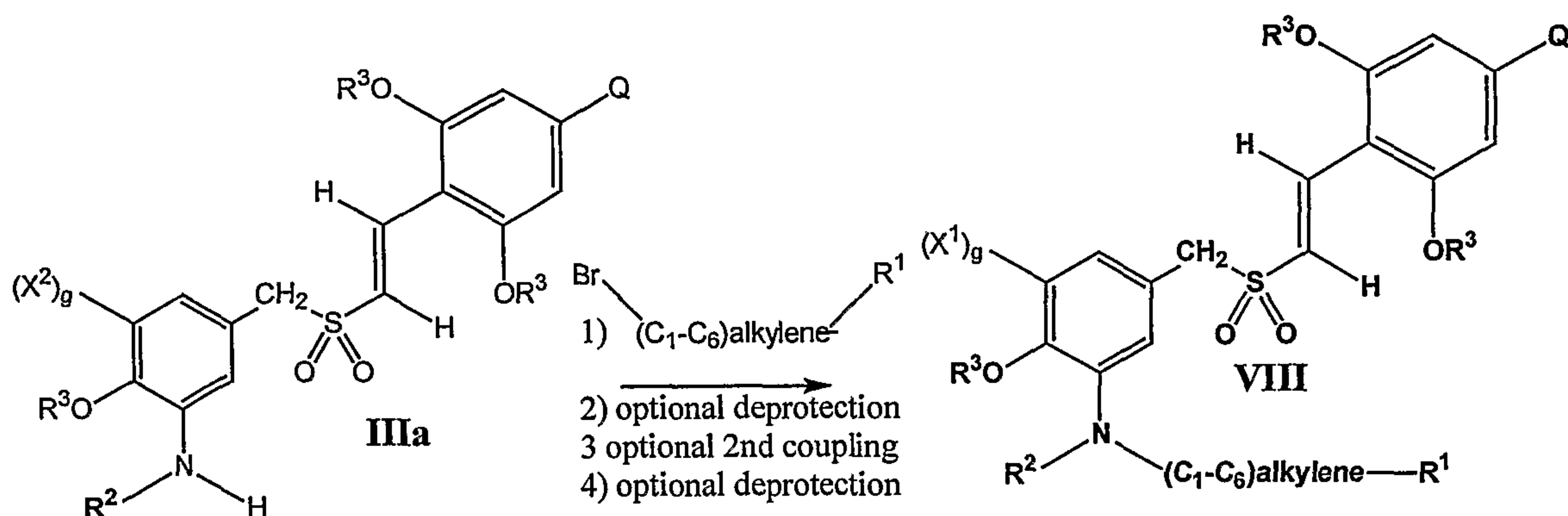
Scheme 6:
