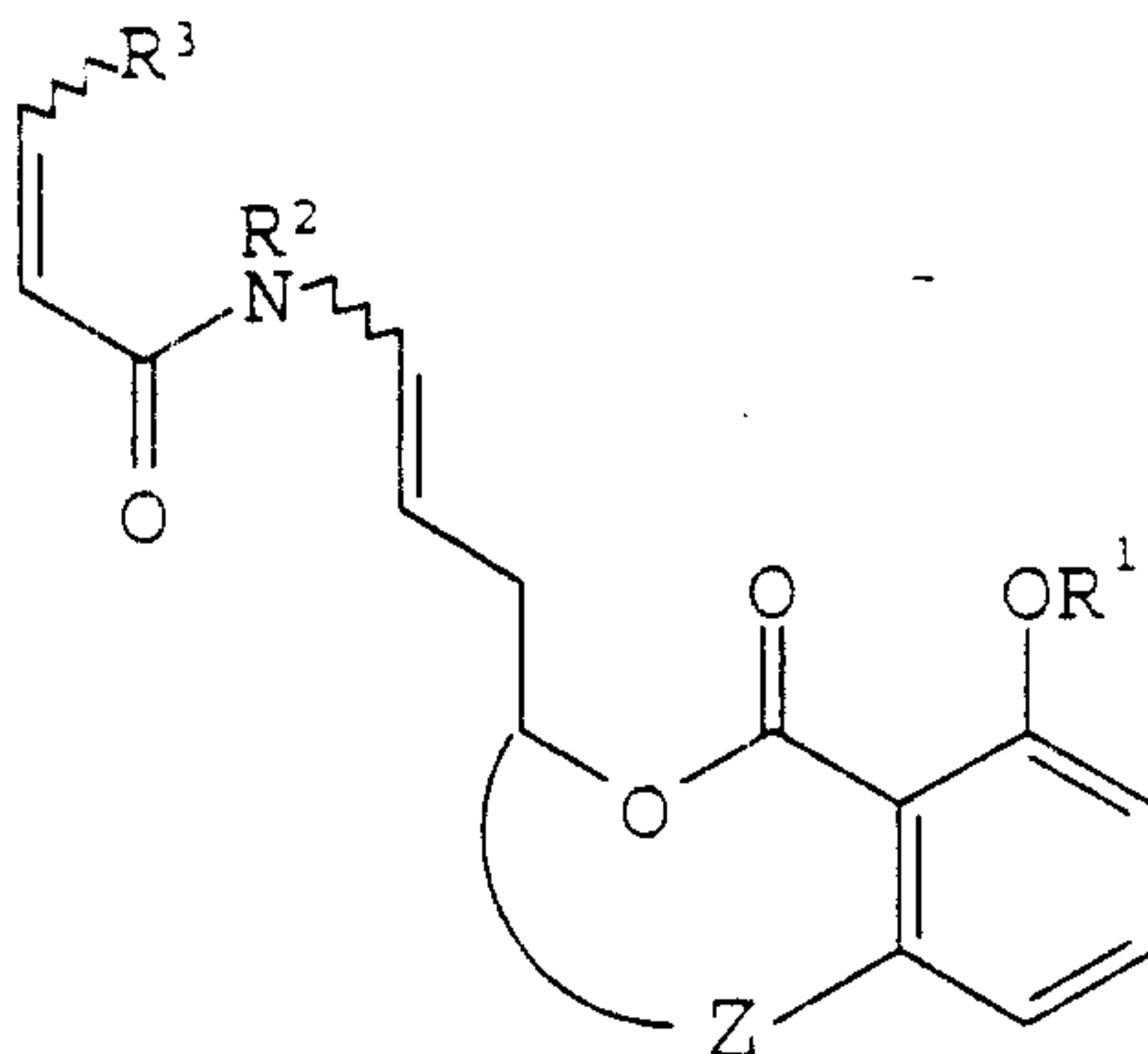
(I)
