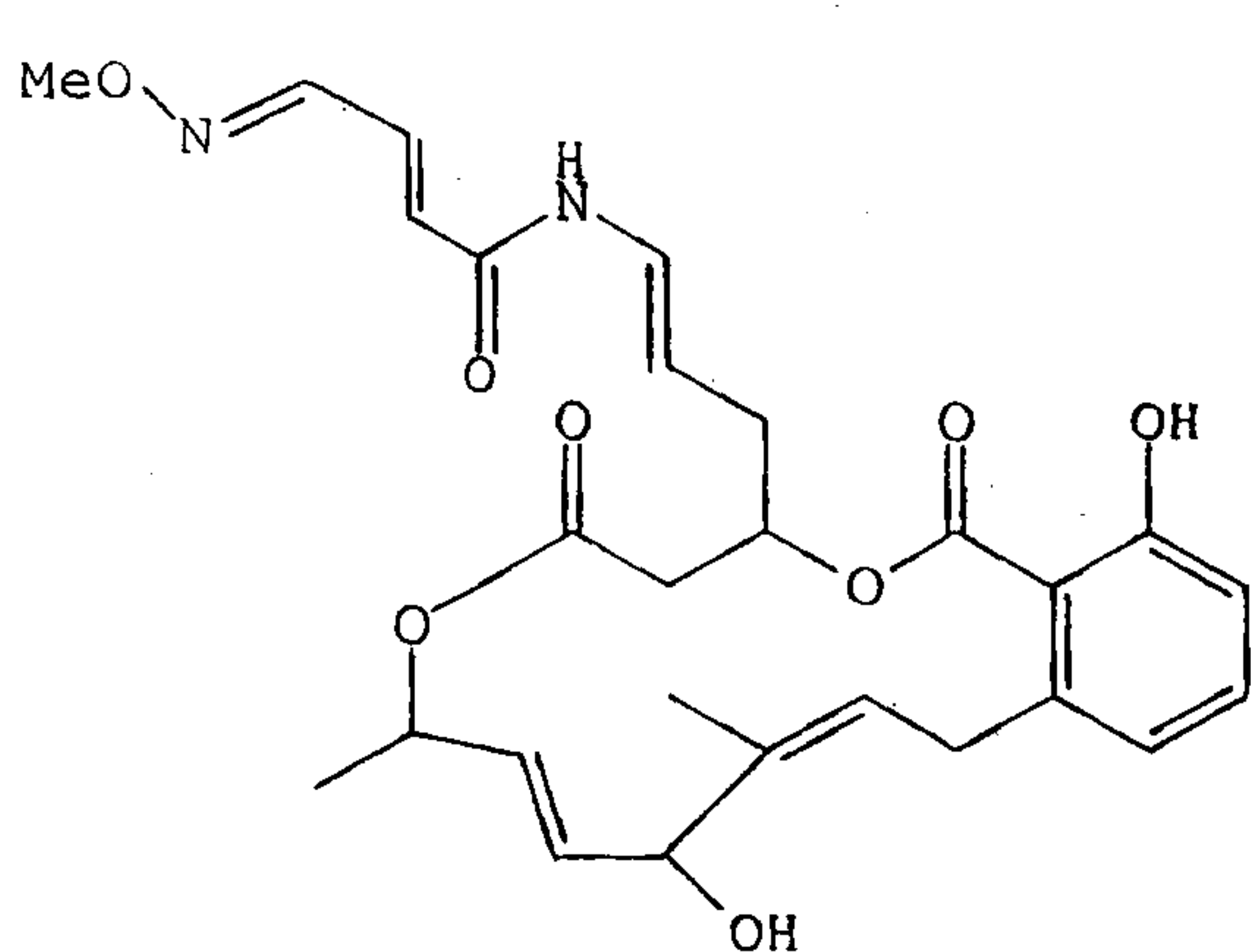
Lobatamide C,
