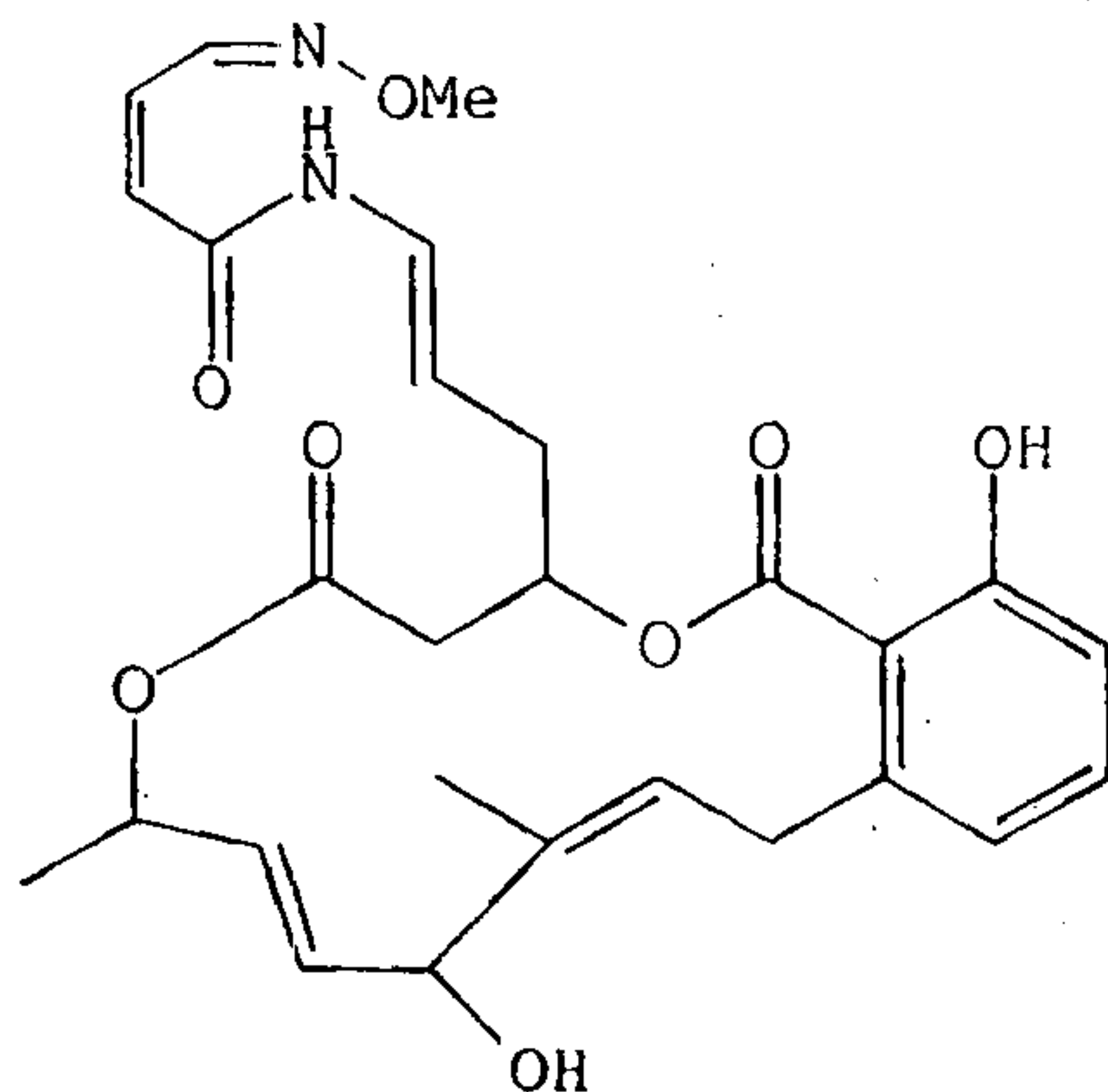
Lobatamide B,
