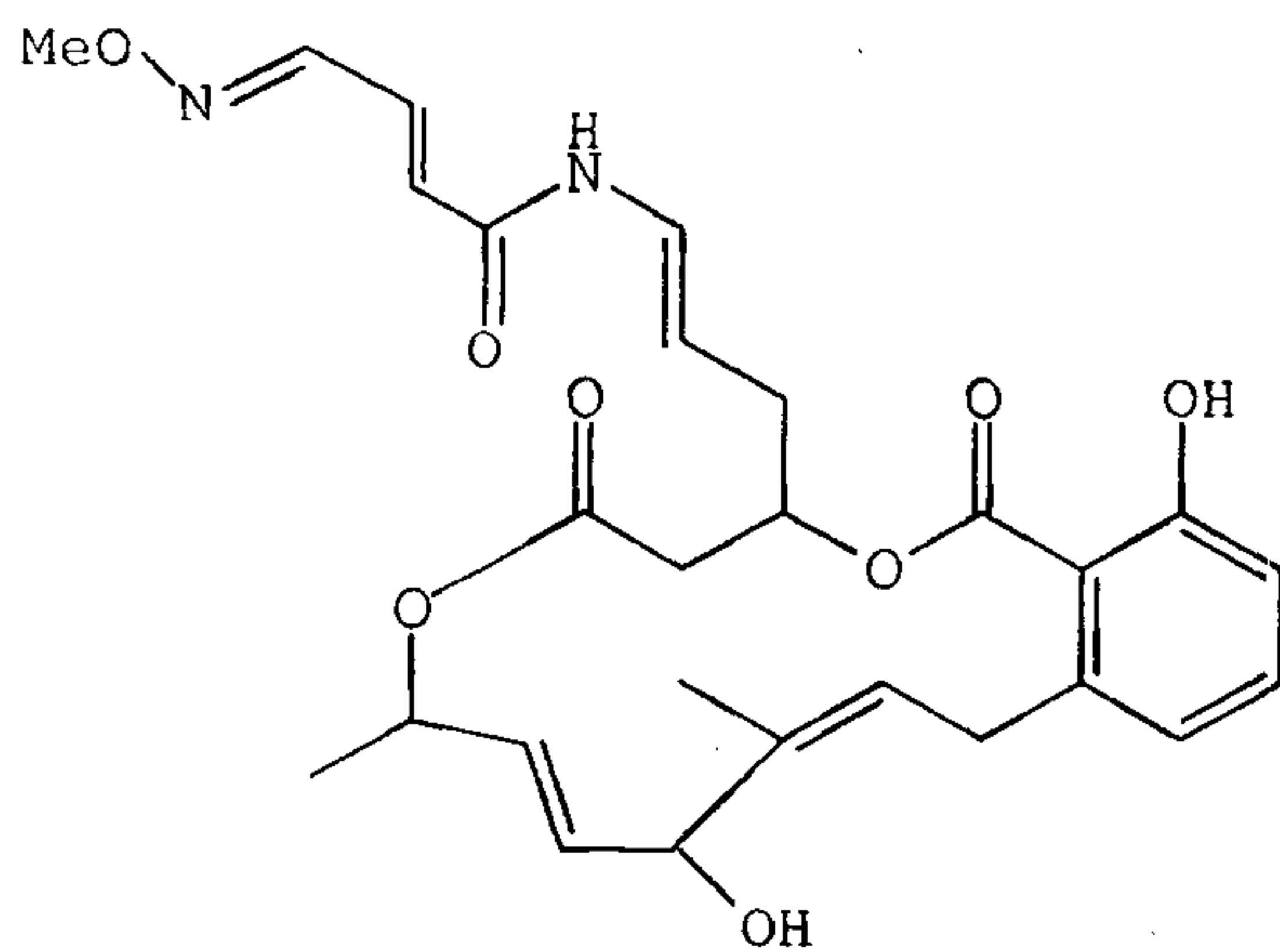
Lobatamide C,
