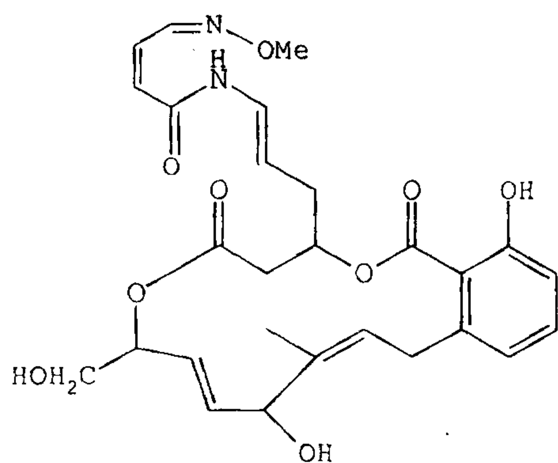
Lobatamide E,
