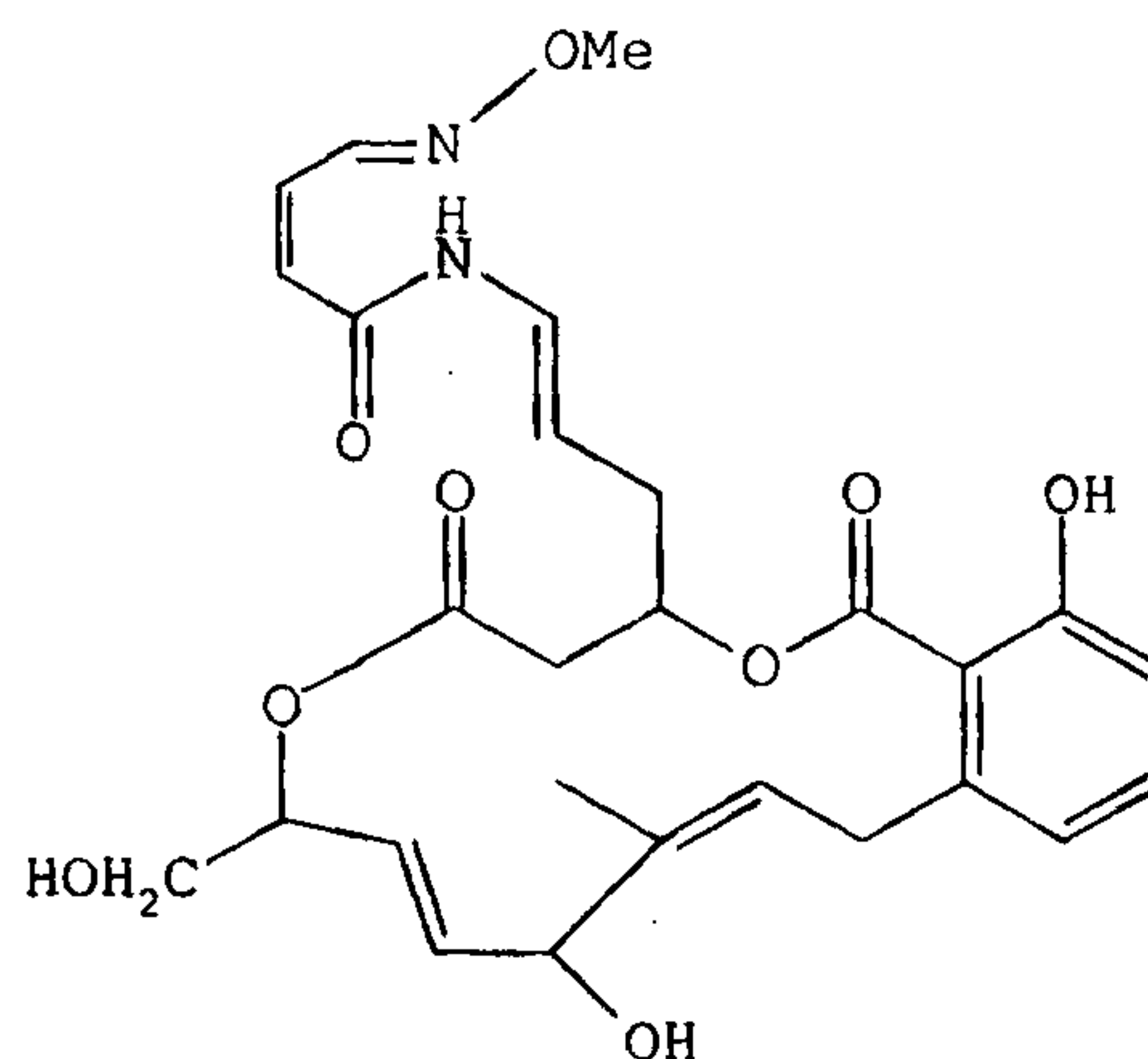
Lobatamide D,
