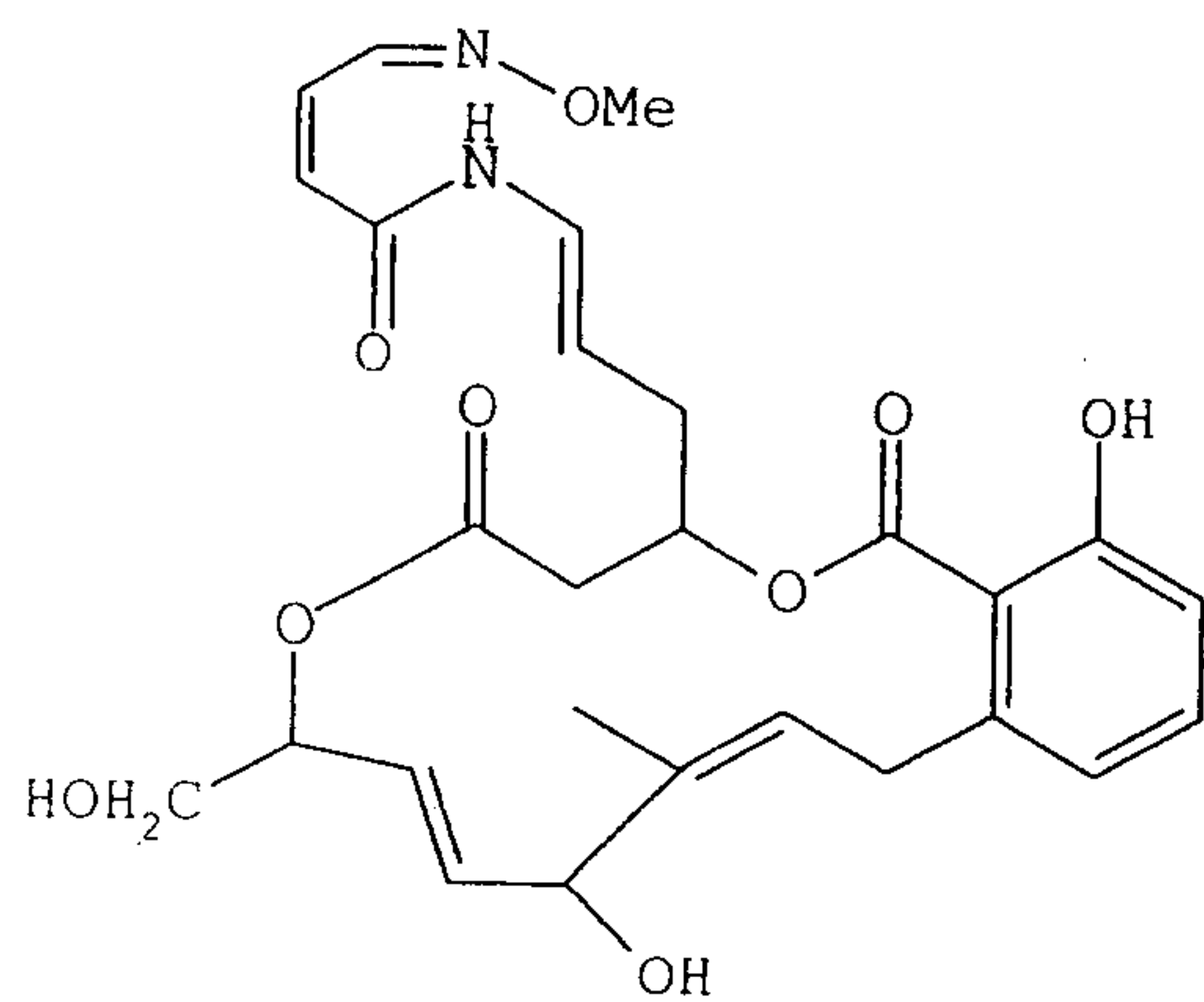
Lobatamide E,
