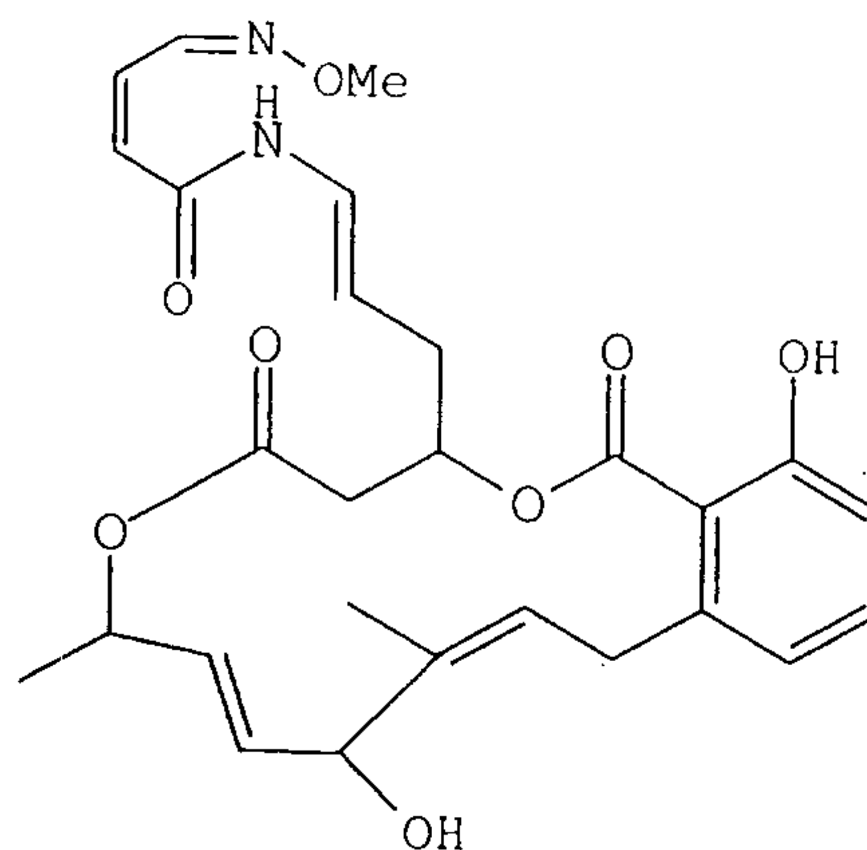
Lobatamide B,
