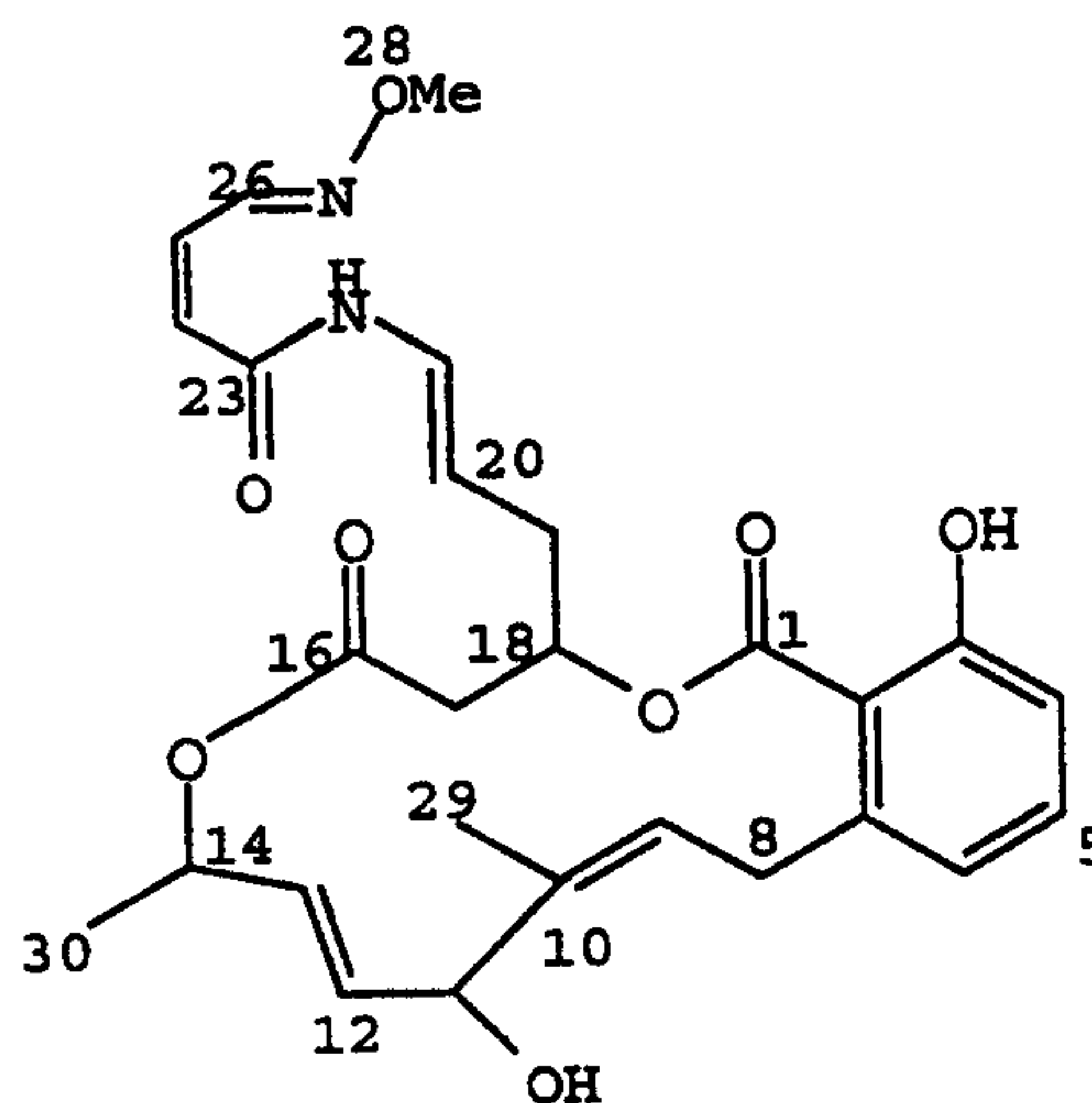
Lobatamide A;
