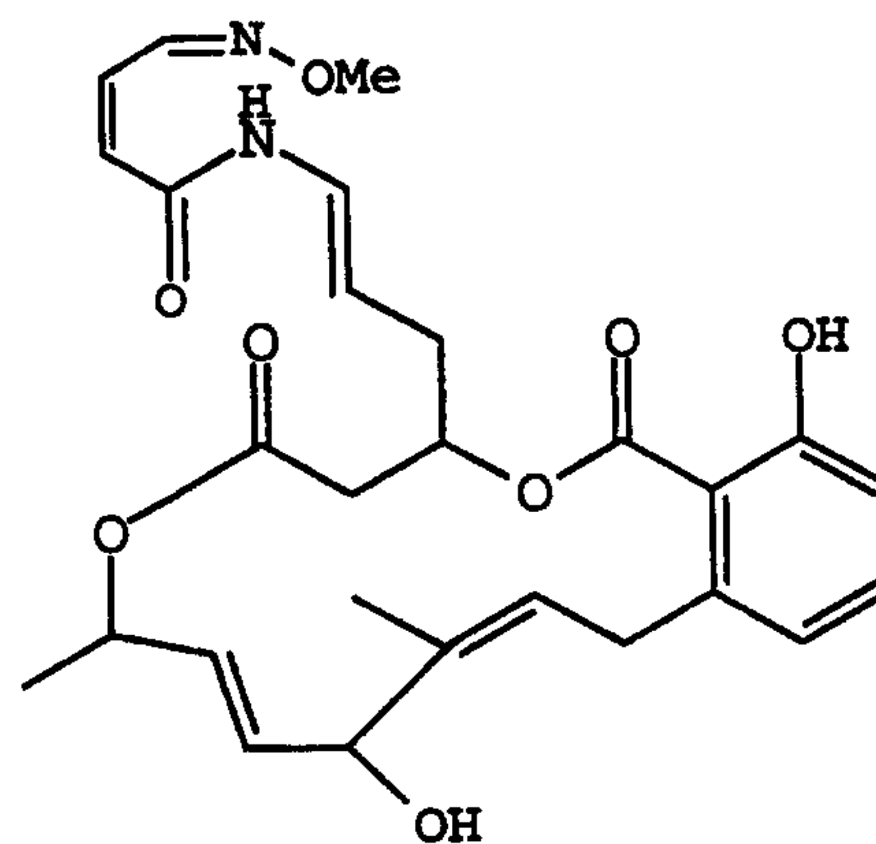
Lobatamide B;
