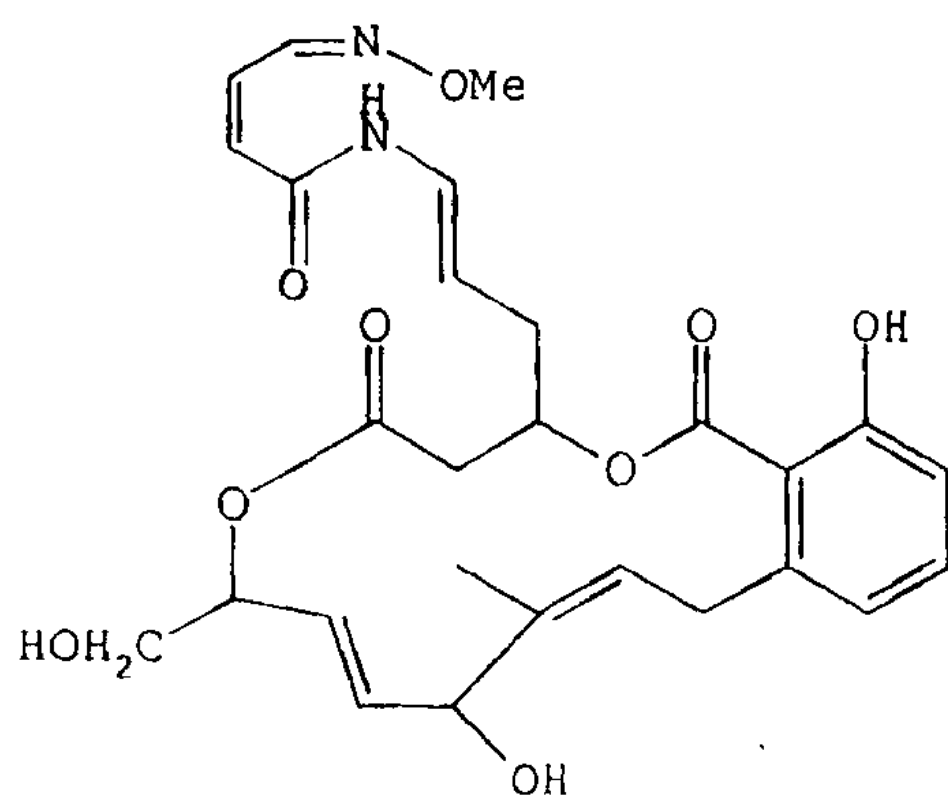
Lobatamide E,
