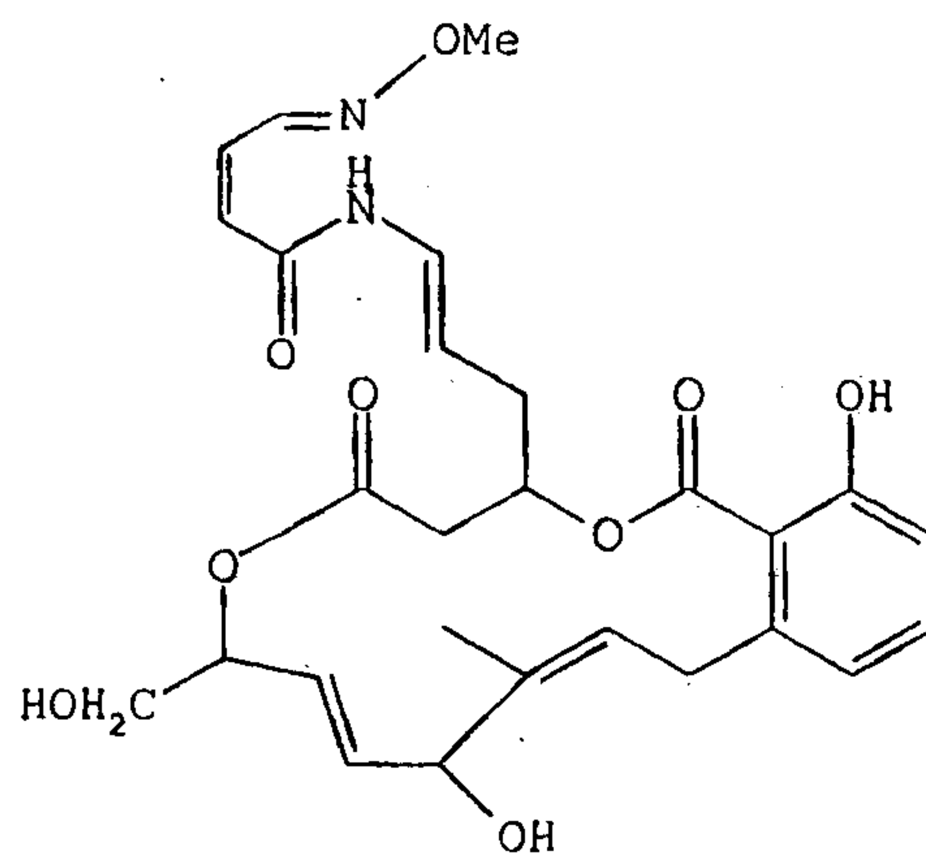
Lobatamide D,
