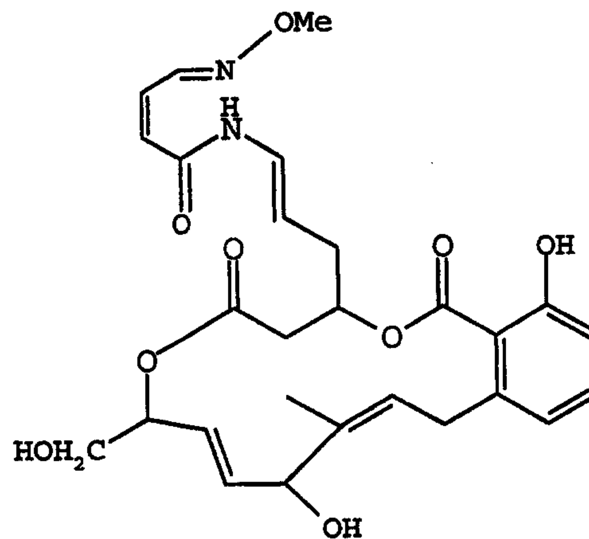
Lobatamide B;
