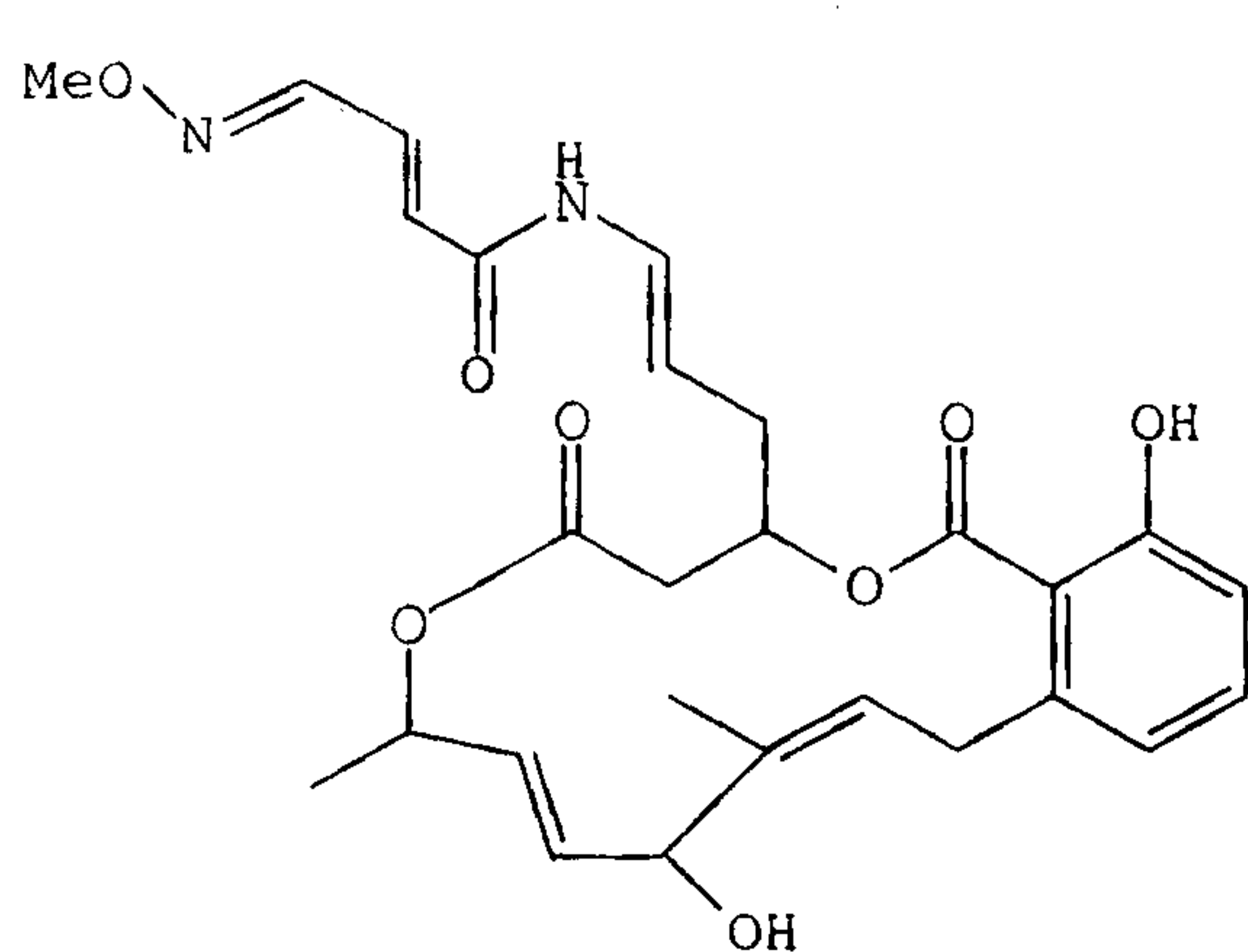
Lobatamide C,
