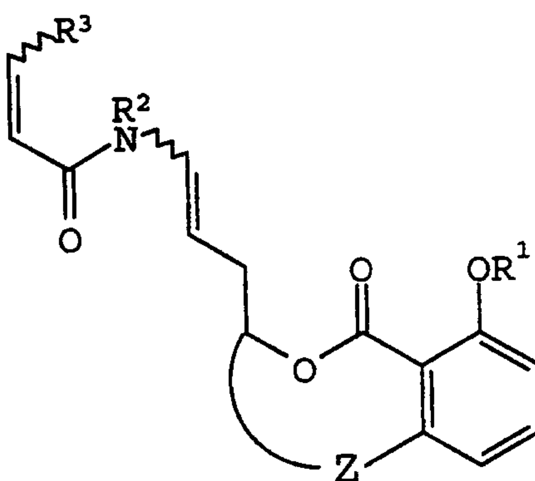
(I)
