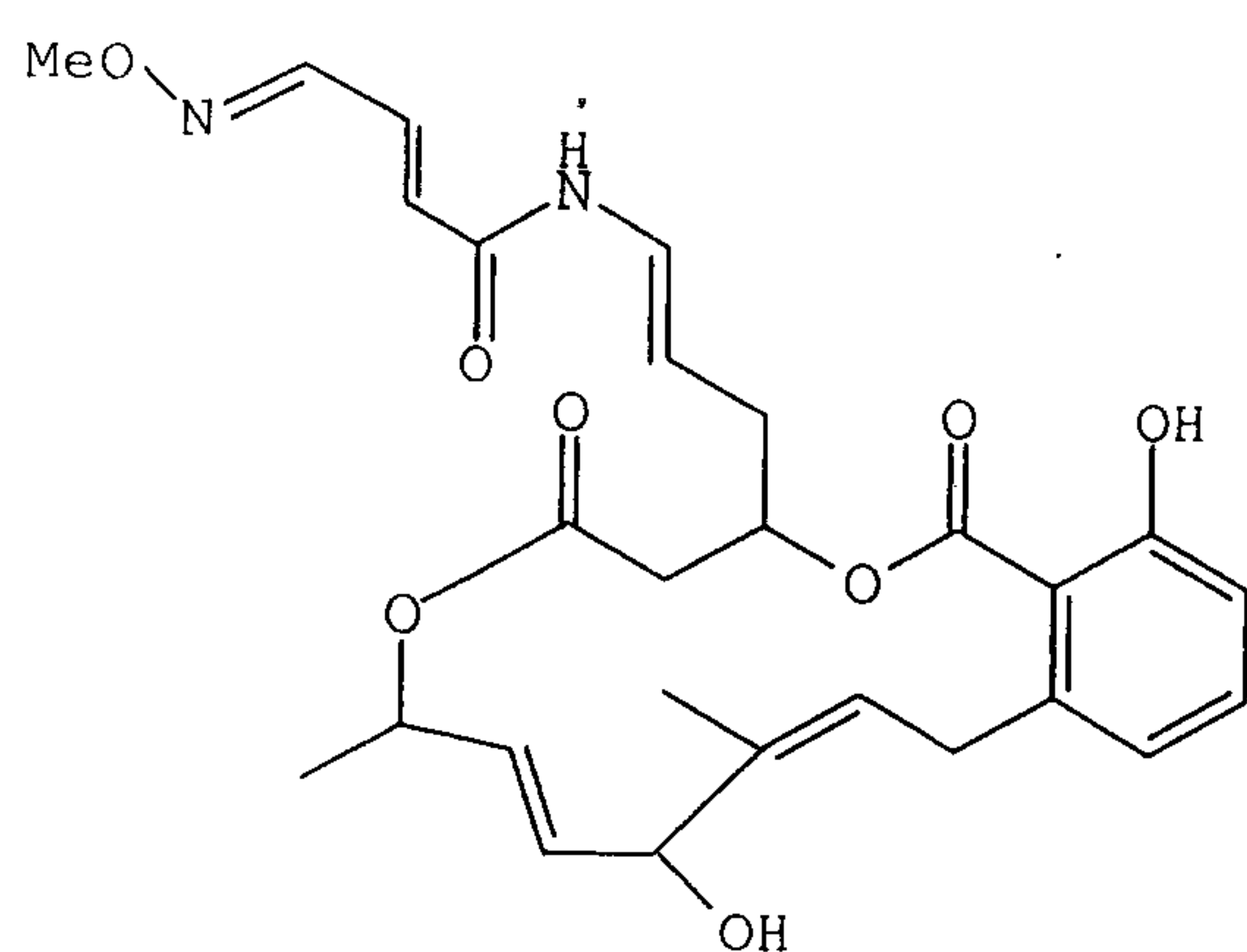
Lobatamide C;
