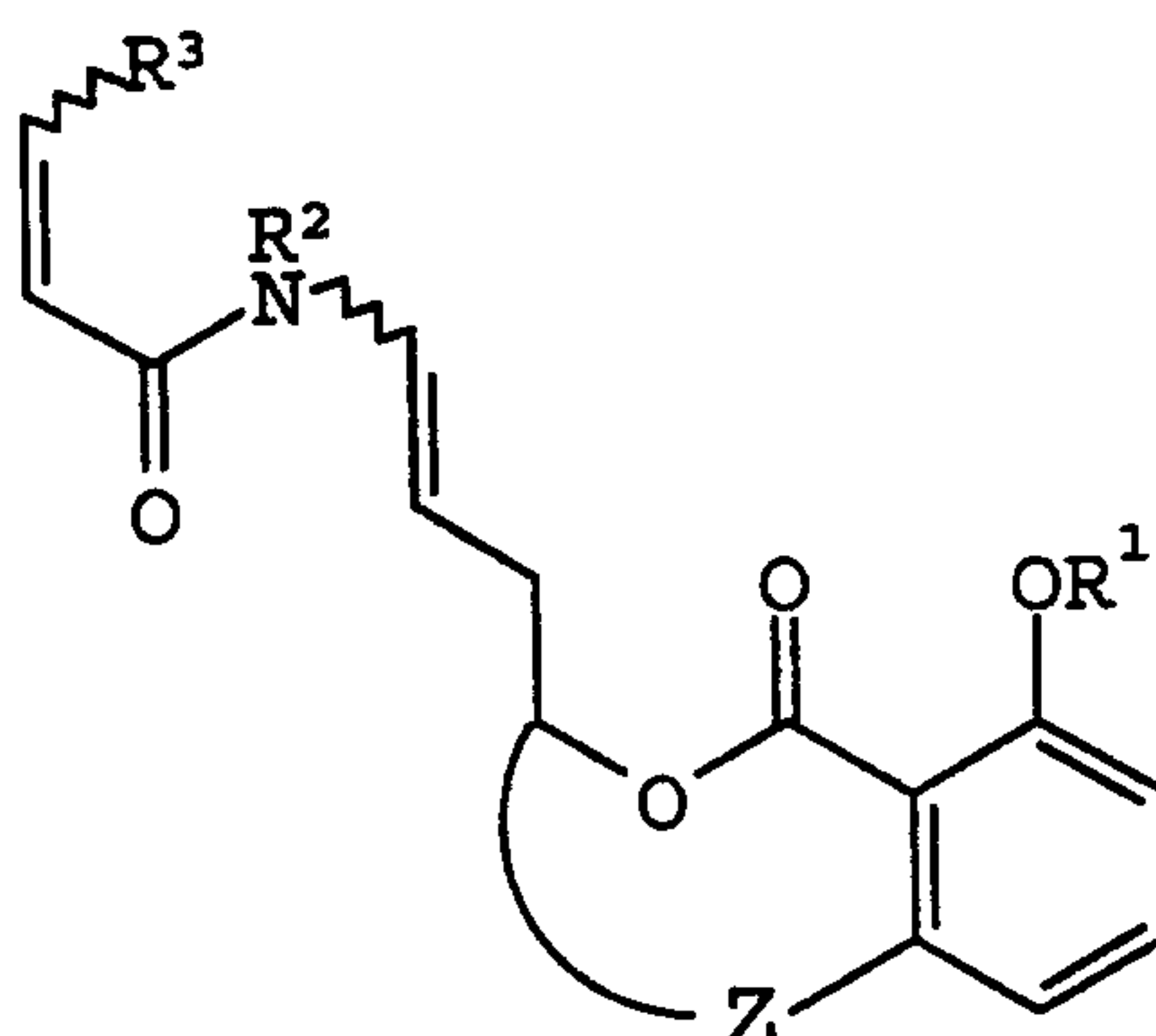
(I)
