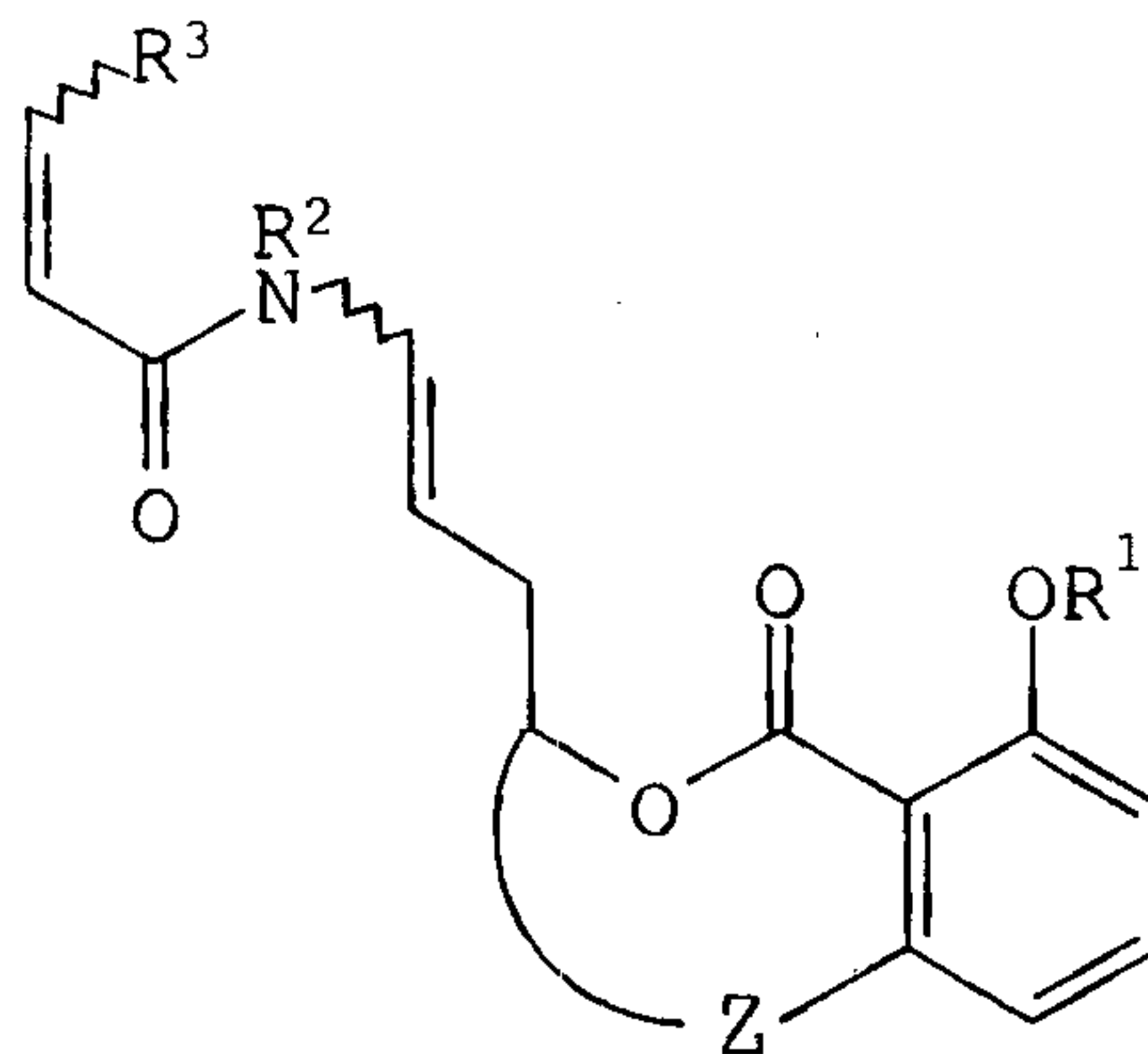
(I),
