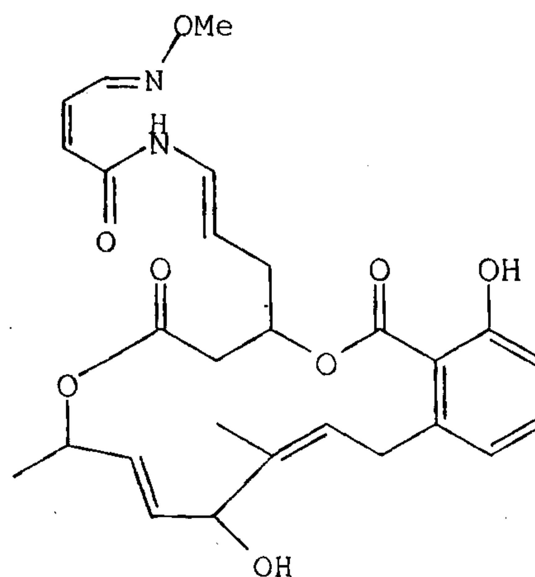
Lobatamide A,
