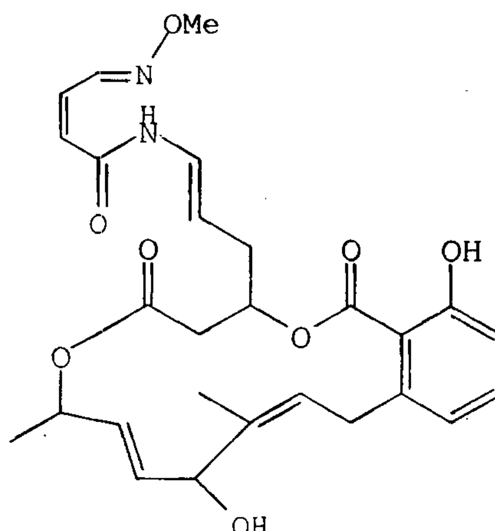
Lobatamide A,
