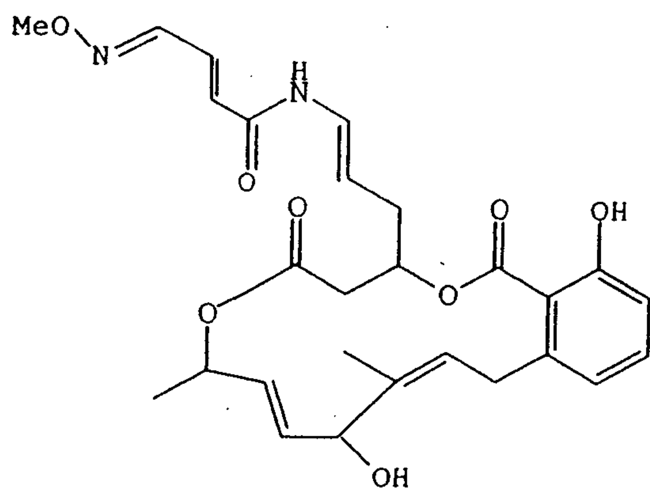
Lobatamide C,
