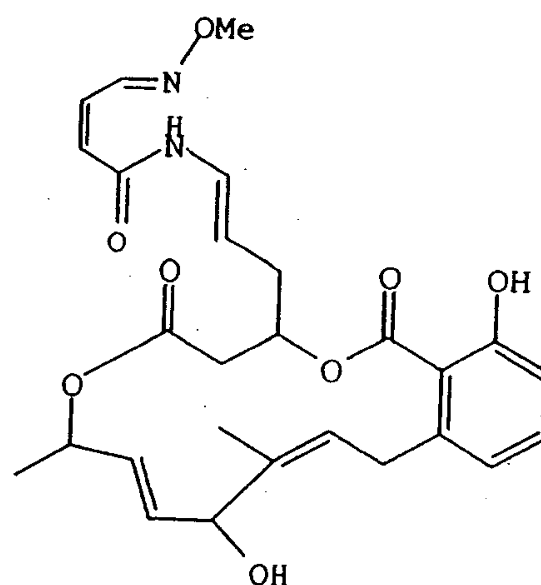
Lobatamide A,
