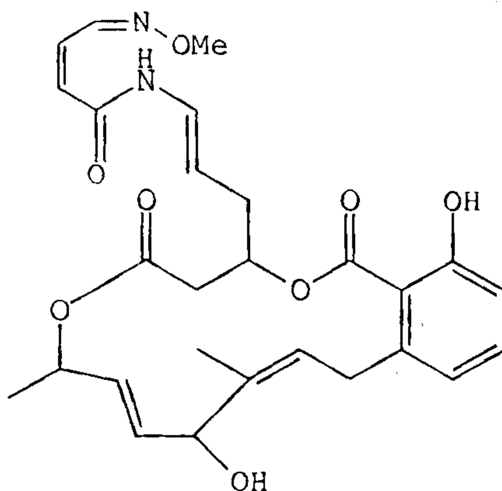
Lobatamide B,
