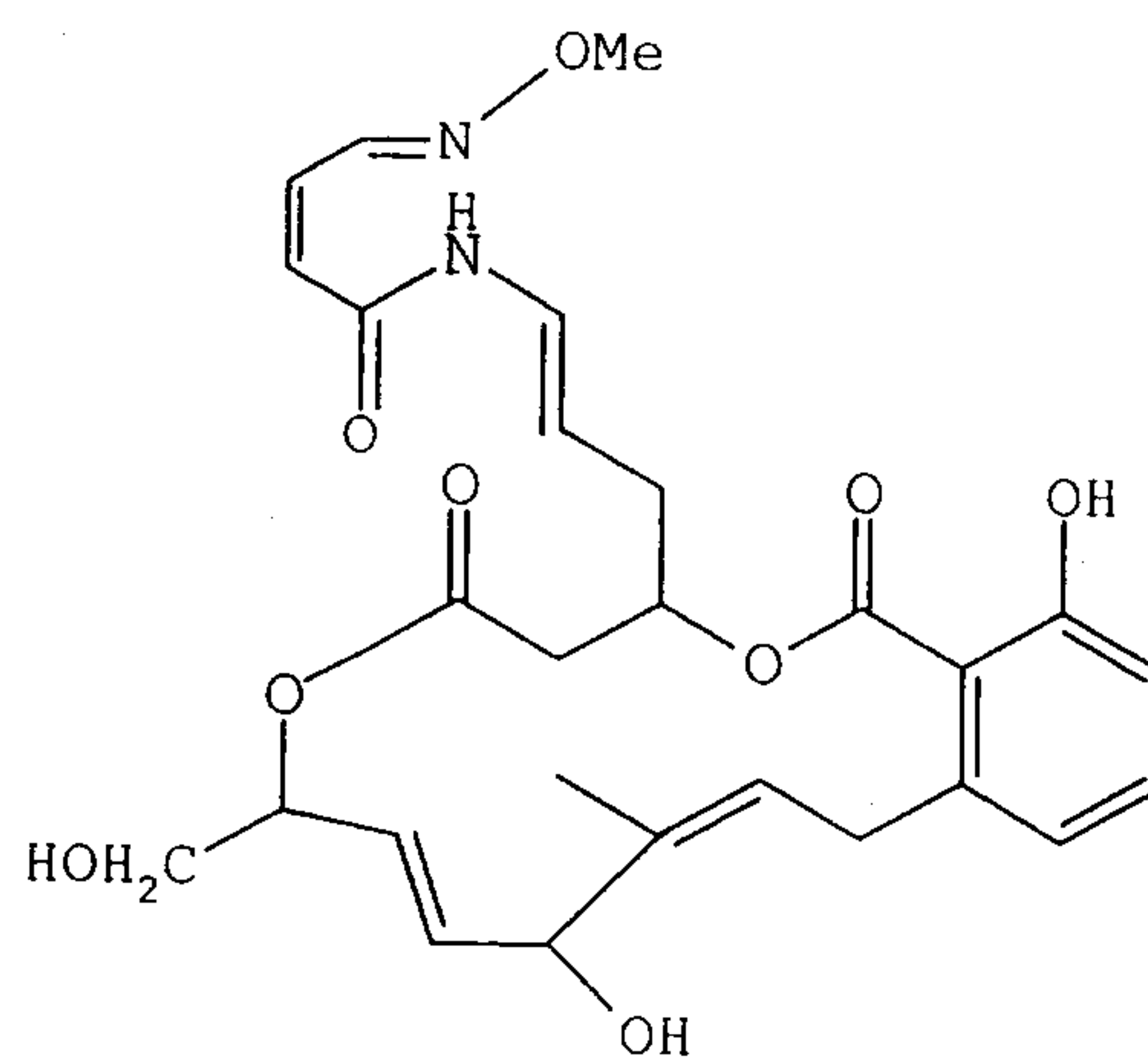
Lobatamide D;
