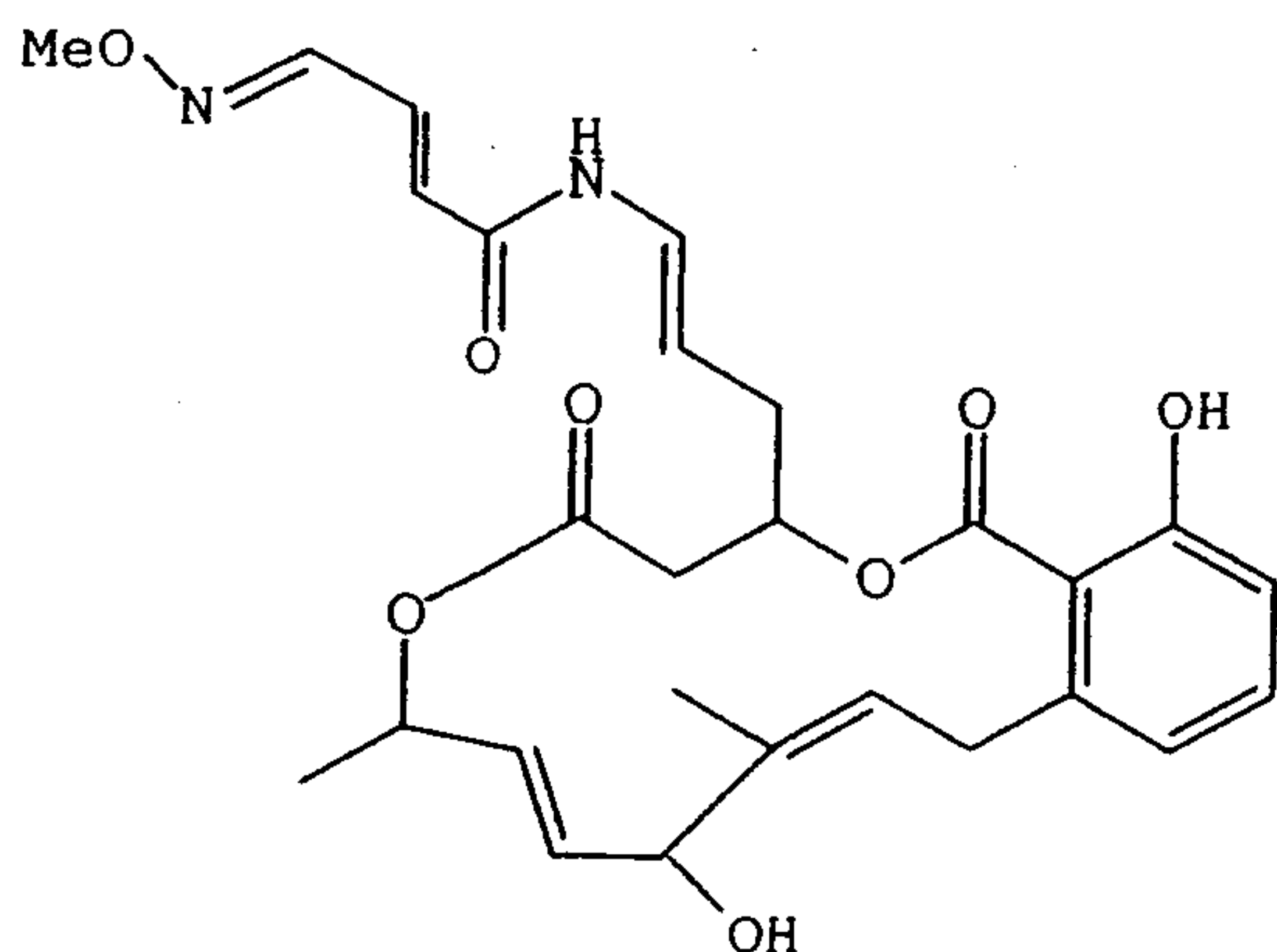
Lobatamide C,
