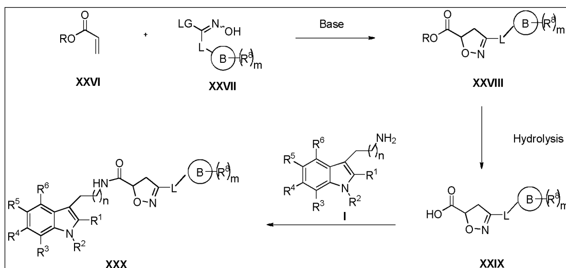
Scheme 7:
