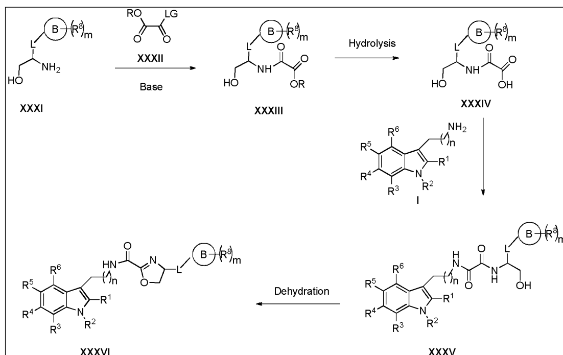
Scheme 8:
