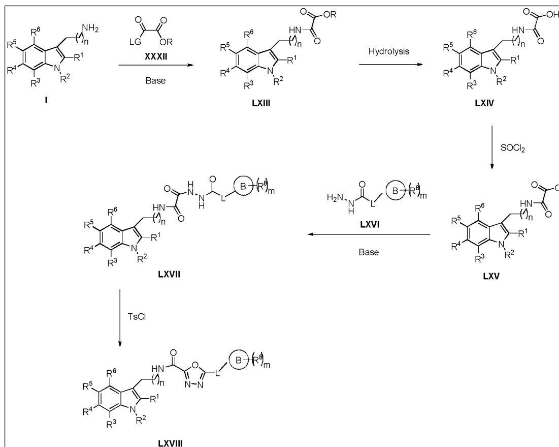
Scheme 15:
