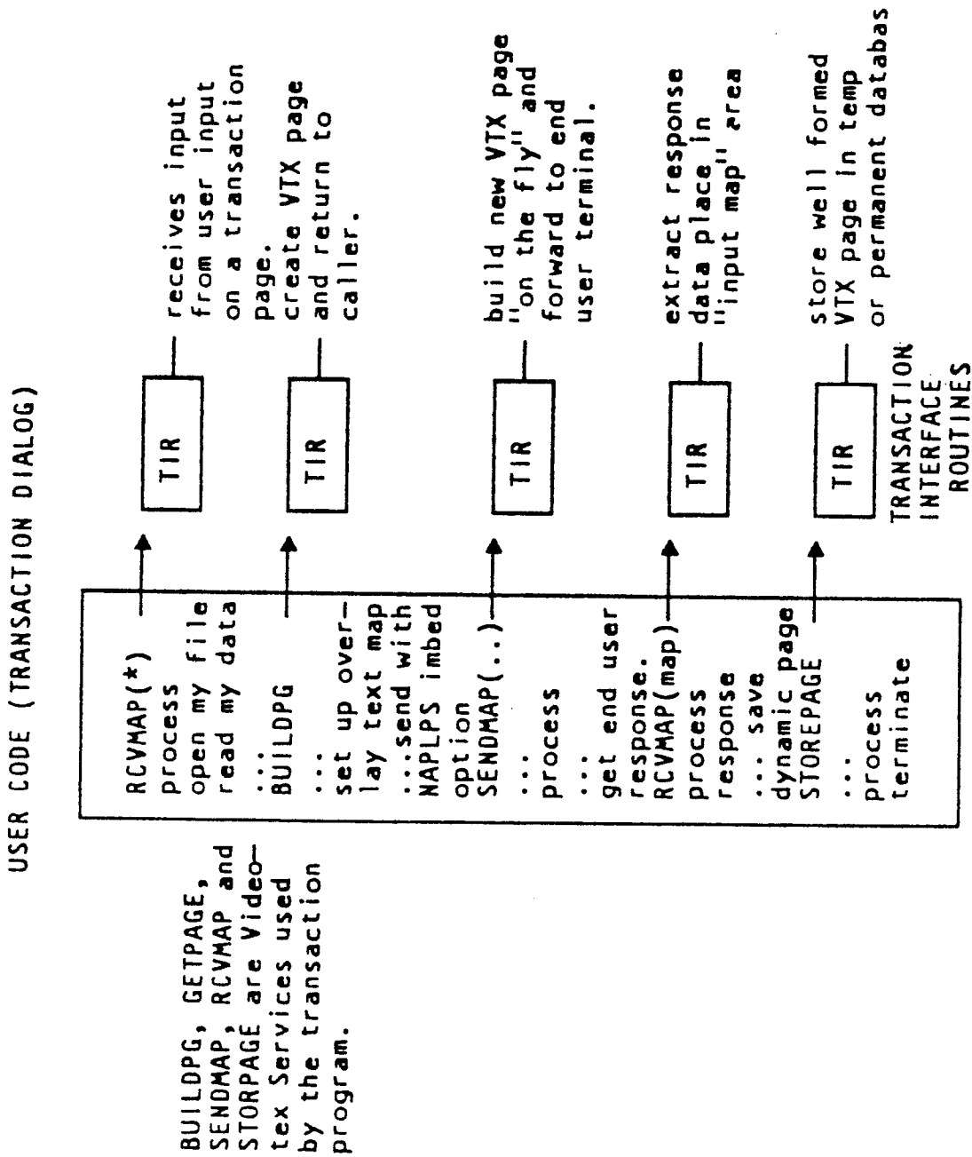
FIG. 7 Sample Transaction Program Outline
