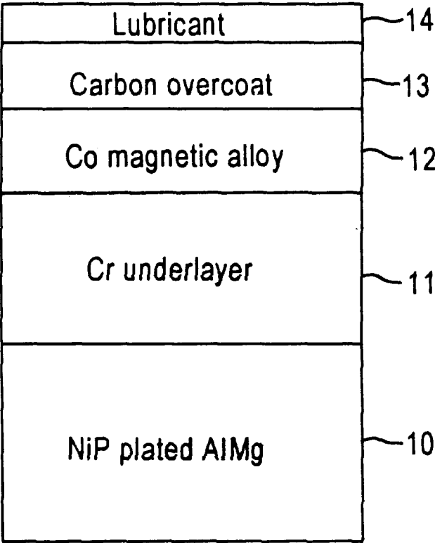
Fig. 1 (PRIOR ART)
