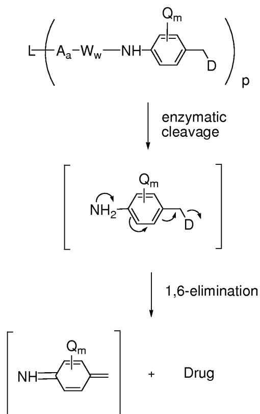
Scheme 3
