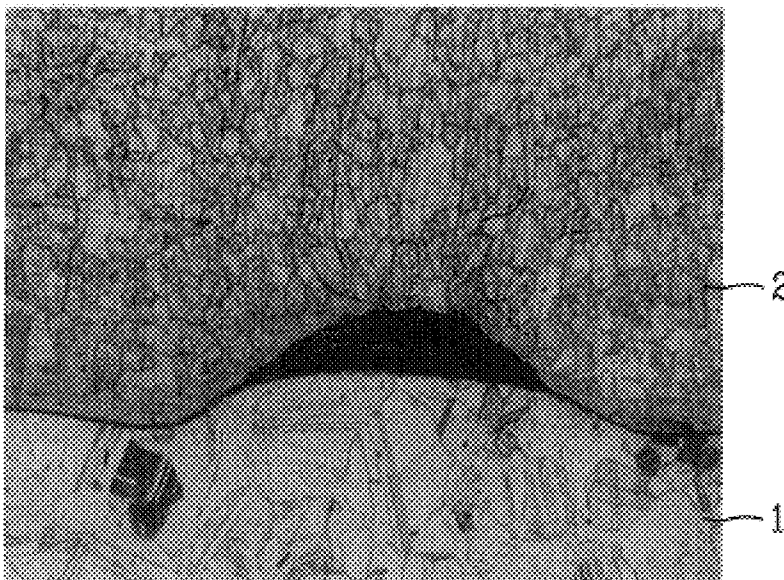
FIG.16 prior art
