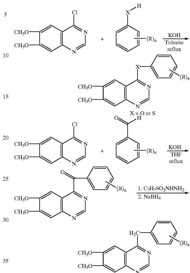
Scheme 3
