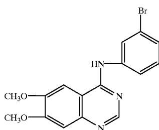
4-(3'-Bromophenyl)-amino-6,7-dimethoxyquinazoline [WHI-P79]
