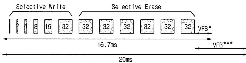
Fig.8 Related Art
