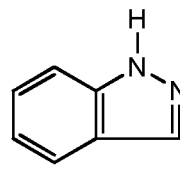
indazole
