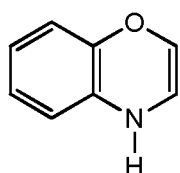
4H-1,4-benzoxazine
