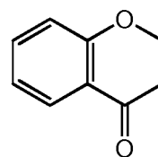
coumarin-4-one (1,4-benzopyrone)
