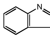
3H-indole (indolenine)
