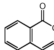
isochromen-1-one (isocoumarin)
