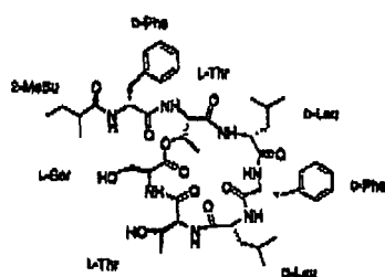
Kahalalide A (1)
