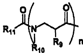
Formula V
