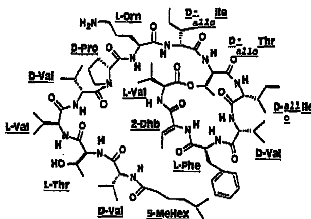
Formula (I)
