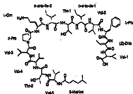
Kahalalide G (7)
