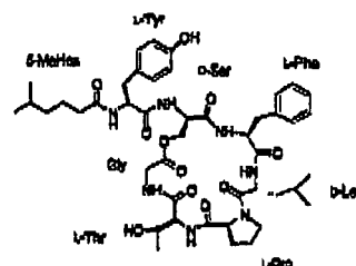
Kahalalide B (2)
