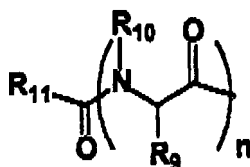
Formula III
