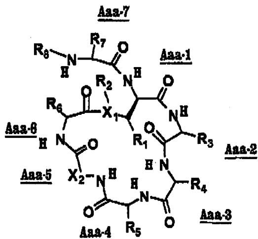
Formula II
