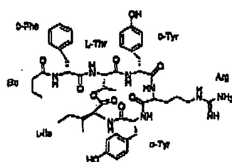
Kahalalide C (3)
