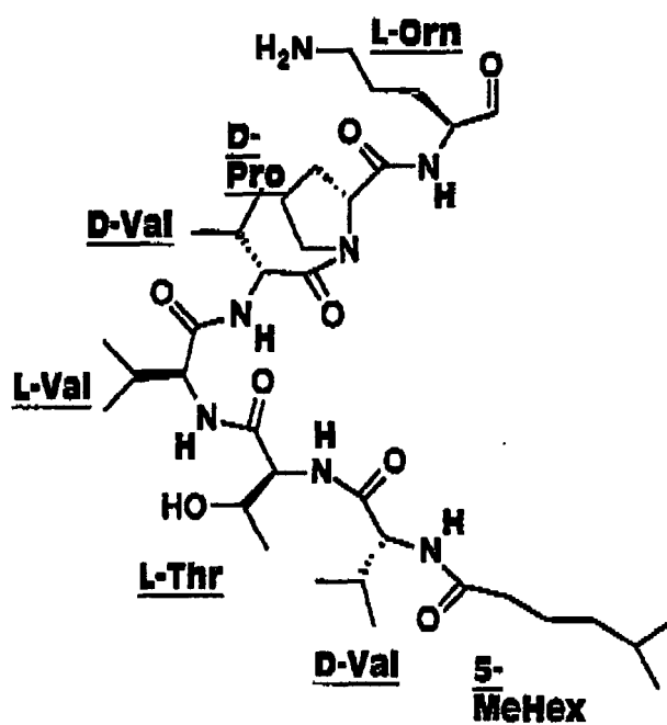
Formula VI
