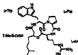
Kahalalide D (4)
