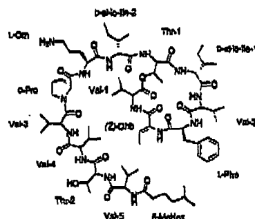
Kahalalide F (6)
