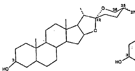
Steroid class
