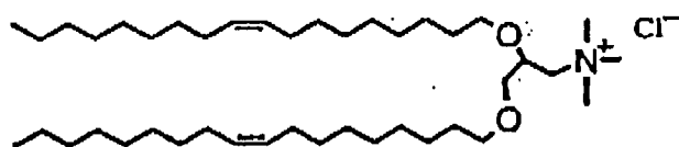
DOTMA
