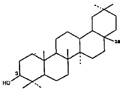
Triterpene class
