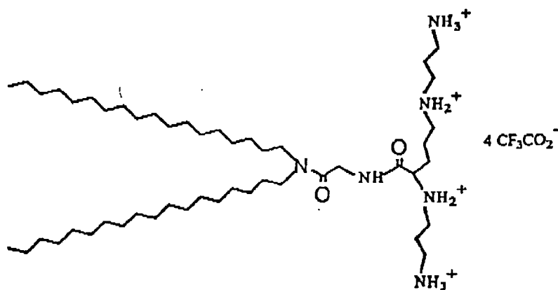
DOGS
