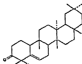
Glutinone (glutinanes)
