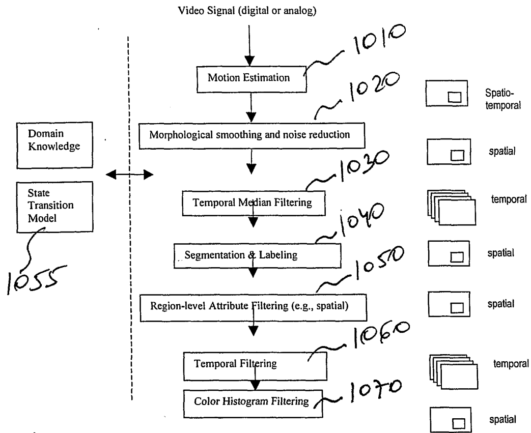
10 Figure 10 Embedded Text Detection Algorithm. The category label (spatial vs. temporal) shown on the right side indicates the domain in which the operation is performed.
