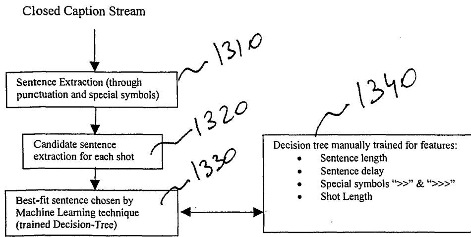
Figure 10 10 Aligning Closed-Captions to video shots 13
