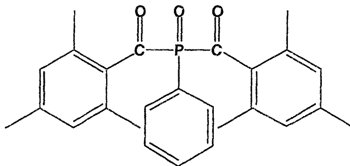
[0040] Figure 1A: Structure of Bis(2,4,6-trimethylbenzoyl)-phenylphosphineoxide
