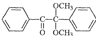
[0042] Figure 1B: Structure of 2,2-dimethoxy-2-phenyl acetophenone (DMPA)
