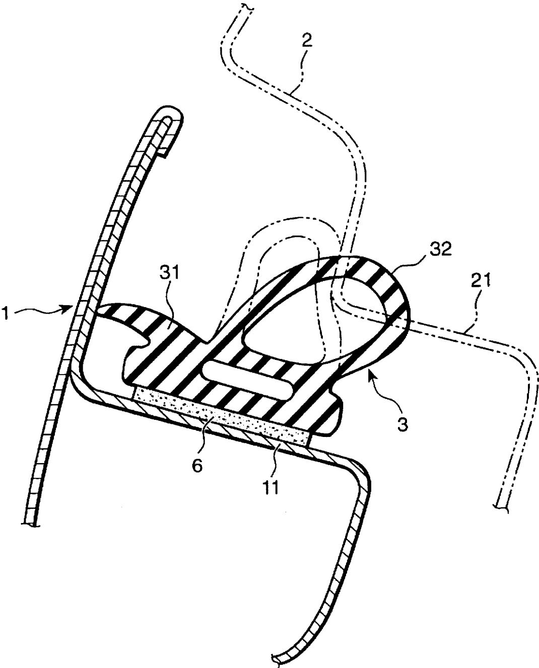
Fig. 4 (PRIOR ART)
