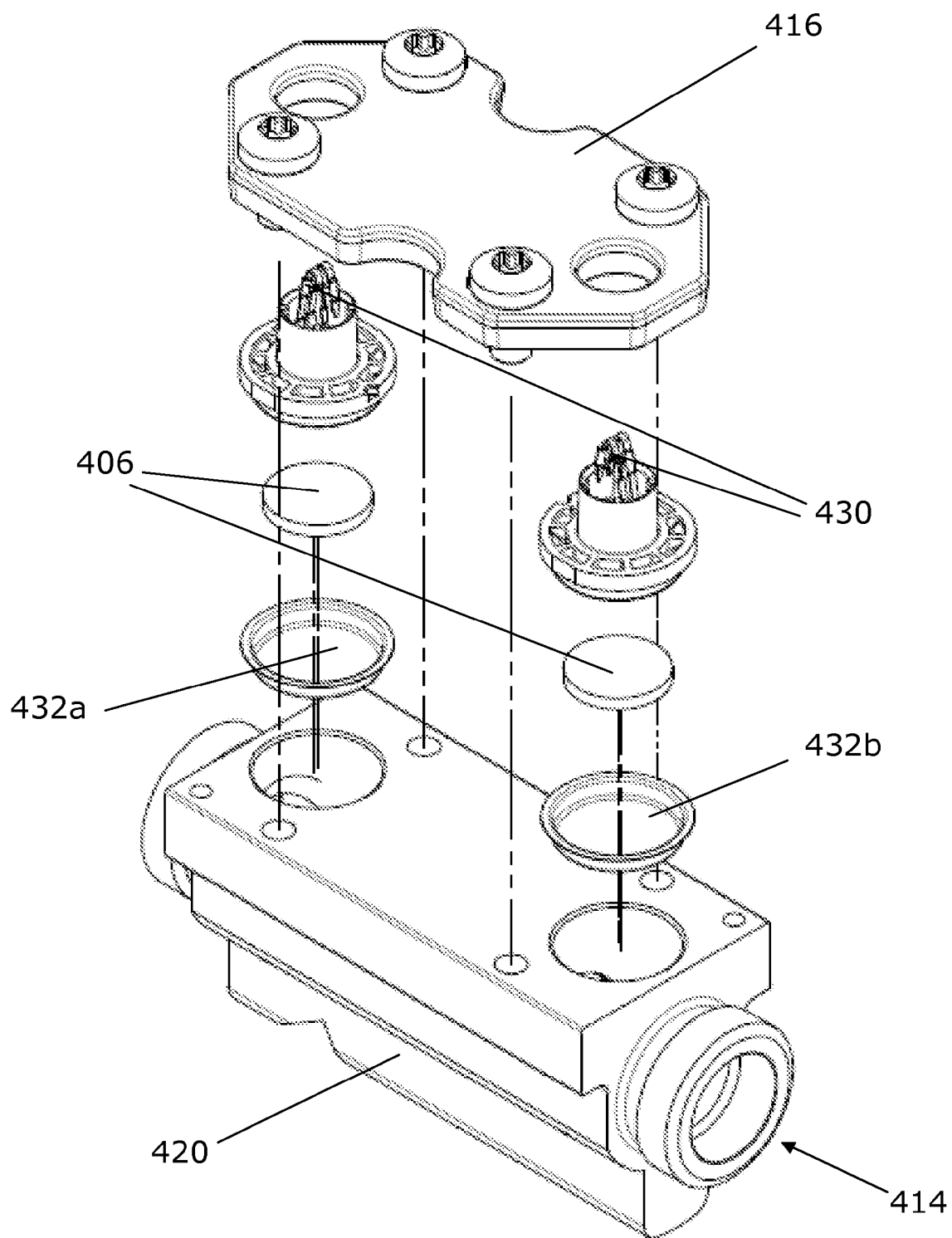
Fig. 4 PRIOR ART
