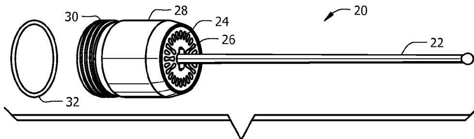
FIG. 2 (Prior Art)
