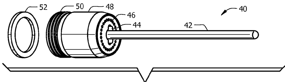
FIG. 3 (Prior Art)
