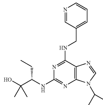
(3S)-3-{(9-Isopropyl-6-[(pyridin-3-ylmethyl)-amino]-9H-purin-2-ylamino)}-2-methyl-pentan-2-ol
