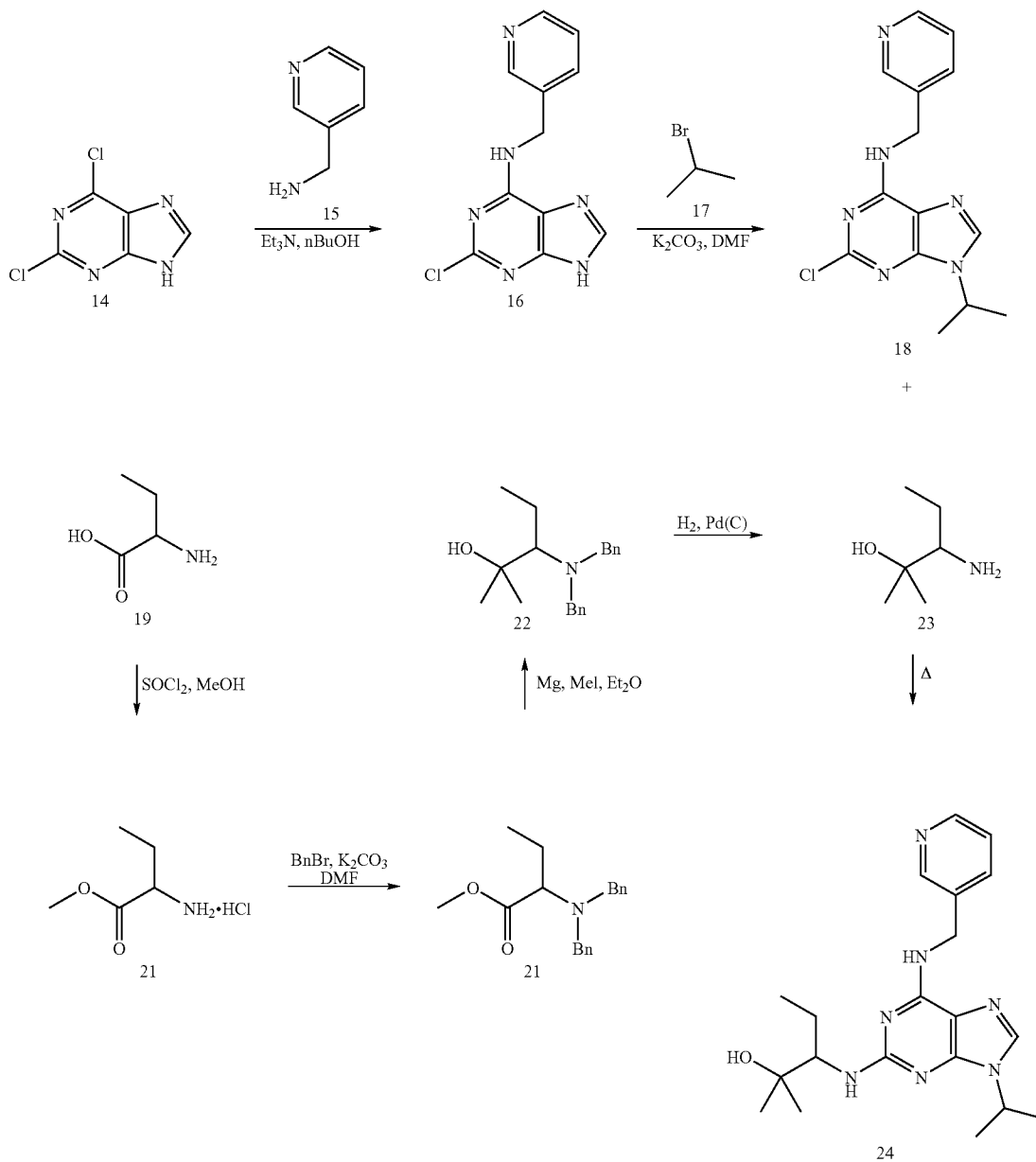
Scheme 3
