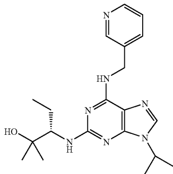
(3R)-3-{(9-Isopropyl-6-[(pyridin-3-ylmethyl)-amino]-9H-purin-2-ylamino)}-2-methyl-pentan-2-ol
