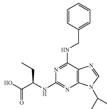
Carboxyl metabolite
