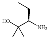
R-3-Amino-2-methyl-pentan-2-ol
