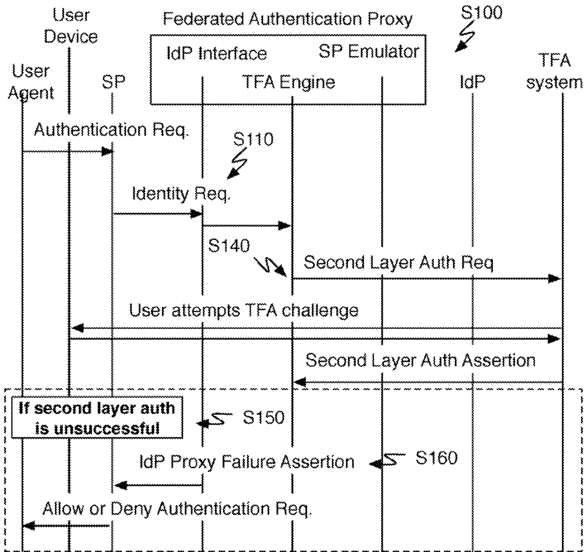
FIGURE 11B
