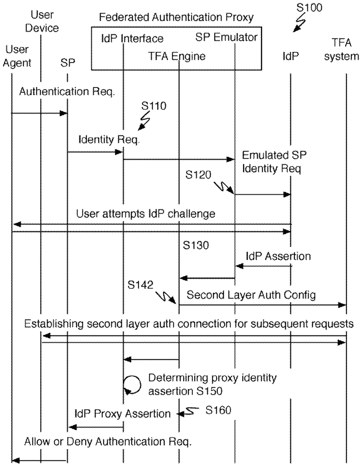
FIGURE 13
