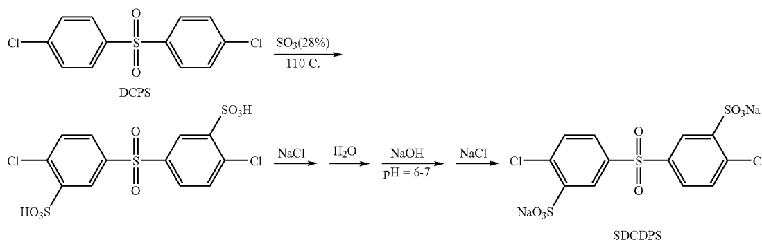
Scheme 4. Synthesis of SDCDPS
