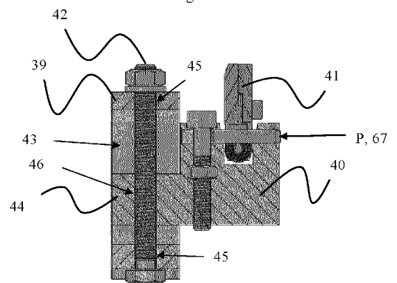
Fig. 9c (Section F-F)
