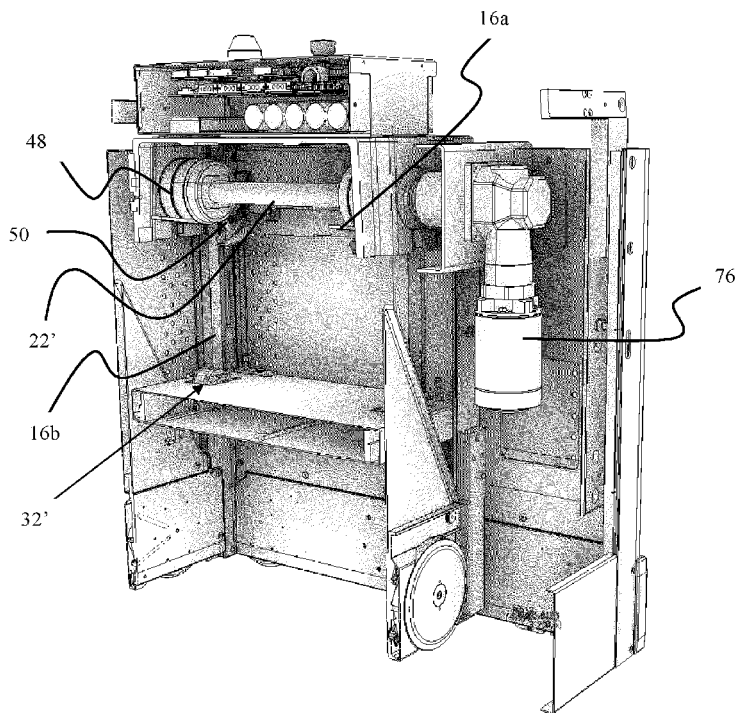
Fig. 25 (Section B-B)
