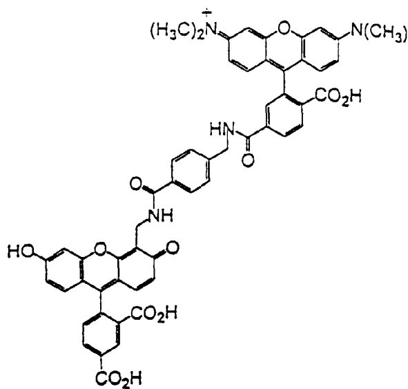
6-TMR-B-CF
