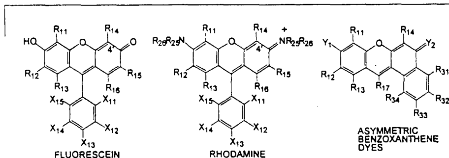
FLUORESCIEIN
