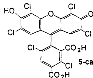
Fluorescein
