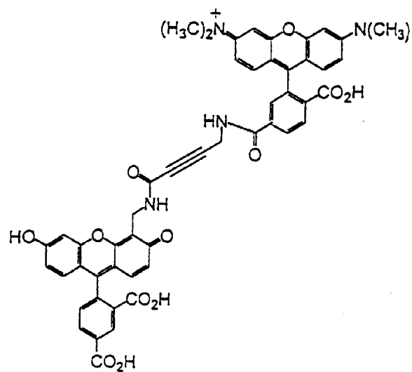
6-TMR-A-CF
