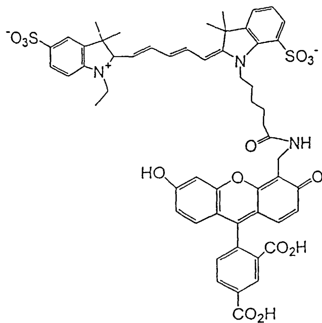
5-ROX-CF
