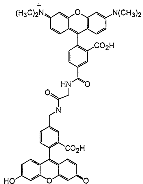
5-TMR-gly-5AMF
