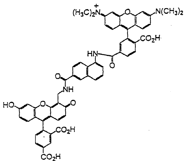
6-TMR-N-CF
