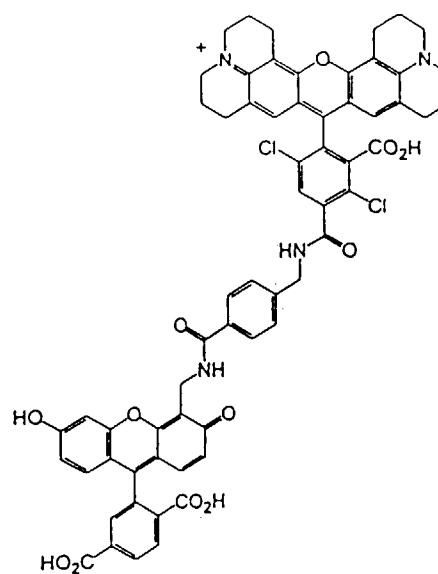
6-CFB-DROX-2
