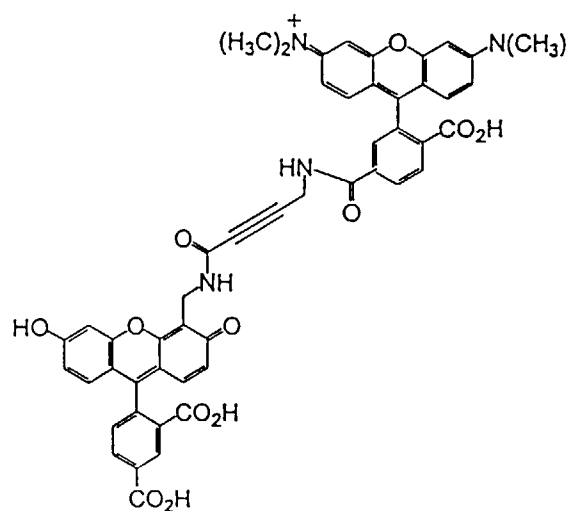
6-TMR-A-CF
