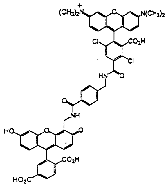
6-CFB-DTMR-2
