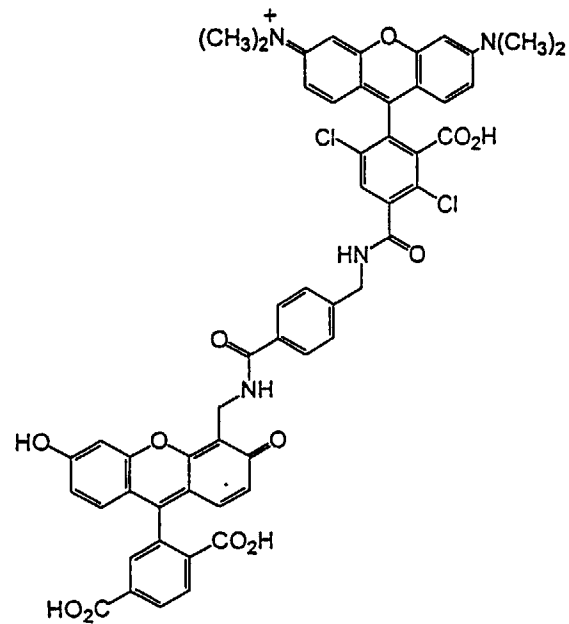
6-CFB-DTMR-2
