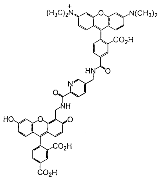
5-TMR-P-CF
