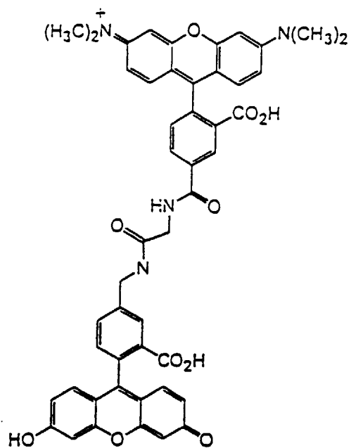
5-TMR-gly-5AMF
