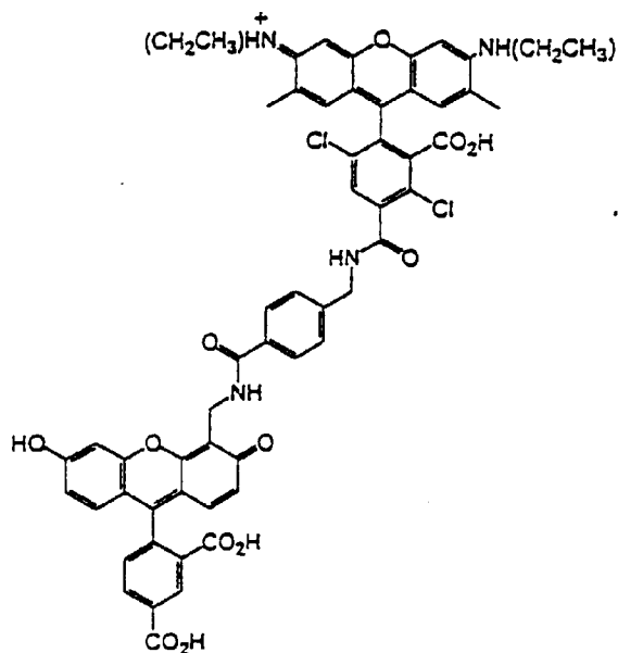
5-CFB-DR6G-2
