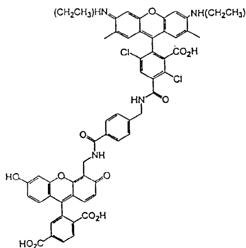
6-CFB-DR6G-2
