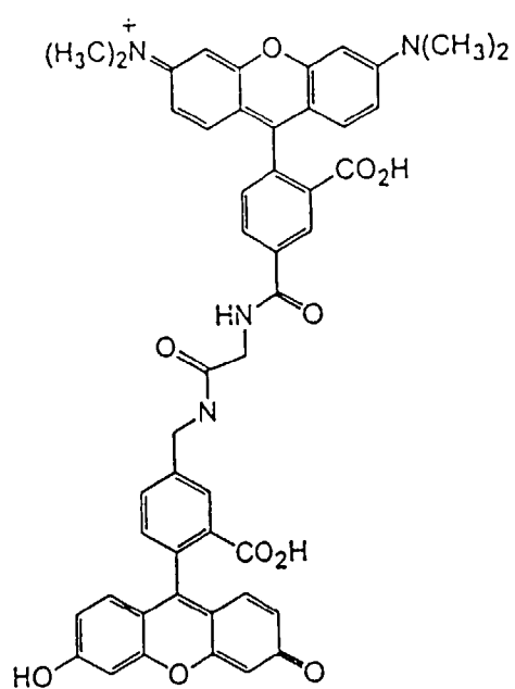
5-TMR-gly-5AMF
