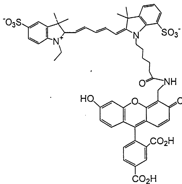
5-ROX-CF
