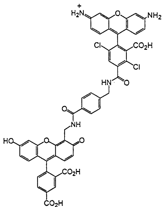
5-CFB-DR110-2
