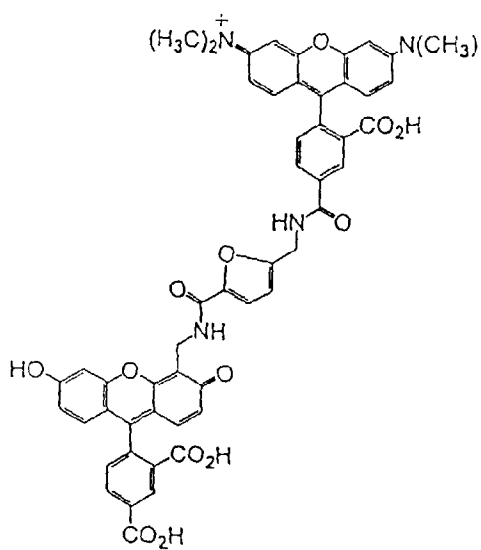
5-TMR-F-CF
