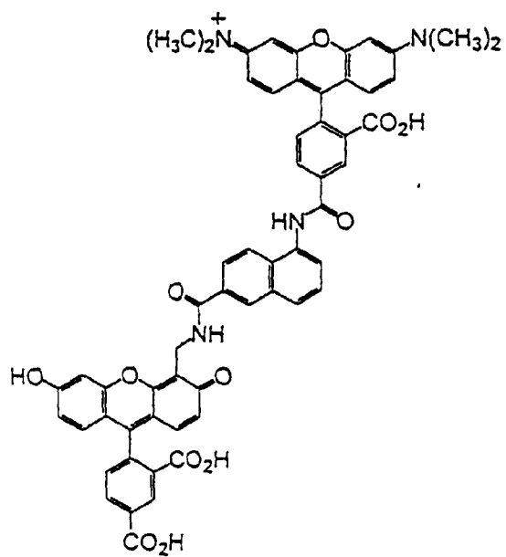
5-TMR-N-CF
