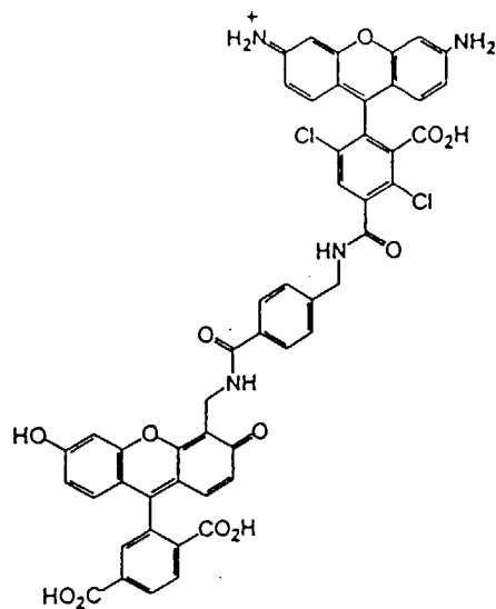
6-CFB-DR110-2
