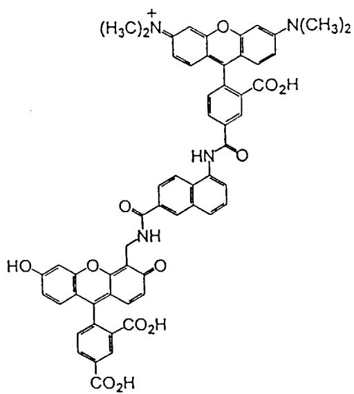
5-TMR-N-CF
