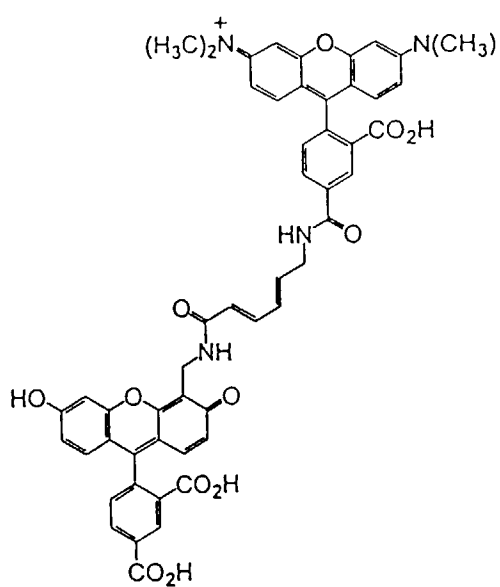
5-TMR-D-CF
