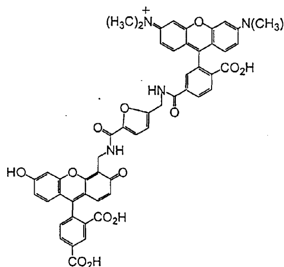
6-TMR-F-CF
