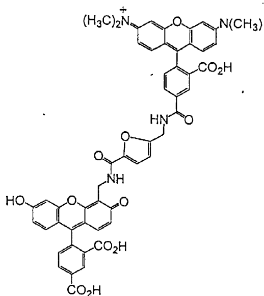
5-TMR-F-CF
