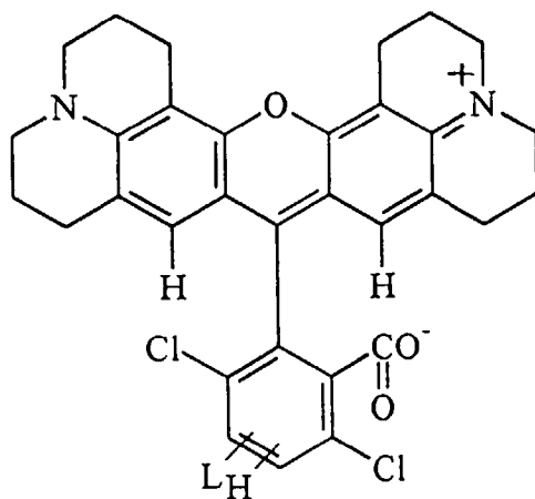
DROX
