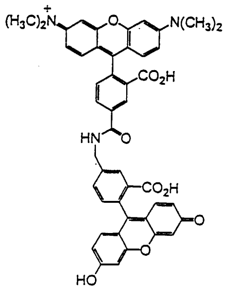
5-TMR-5AMF
