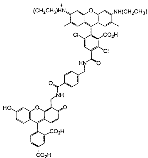
5-CFB-DR6G-2
