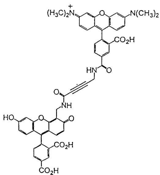
5-TMR-A-CF
