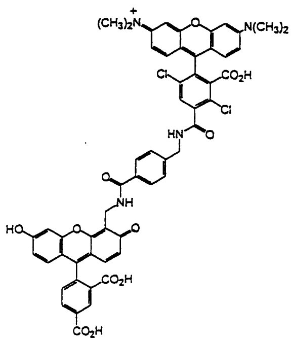
5-CFB-DTMR-2
