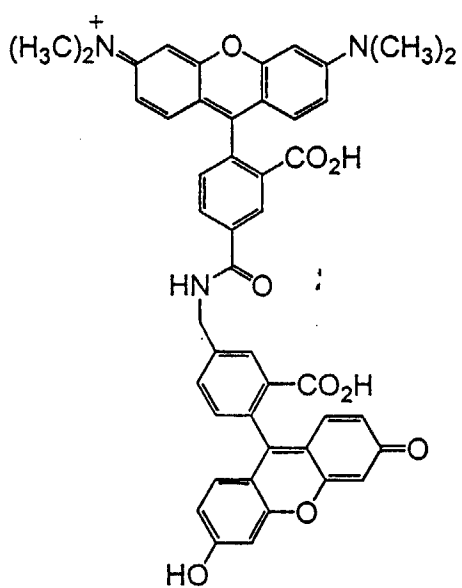
5-TMR-5AMF
