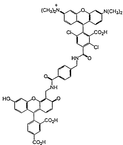
5-CFB-DTMR-2
