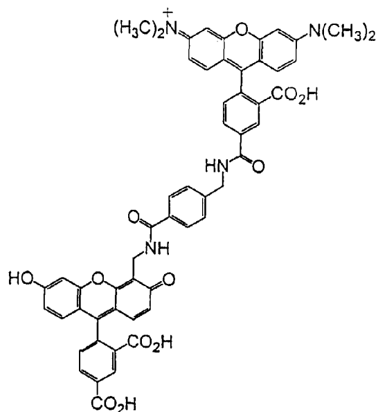
5-TMR-B-CF
