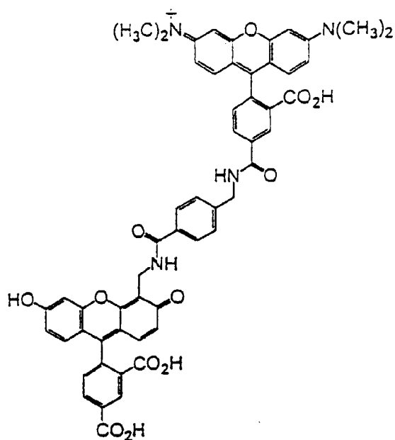
5-TMR-B-CF
