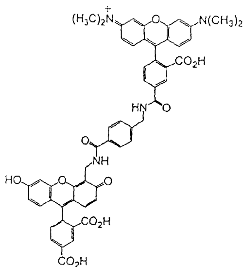
5-TMR-B-CF
