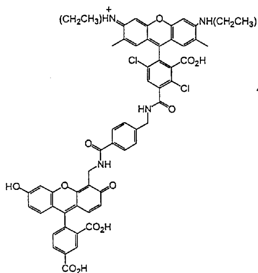
5-CFB-DR6G-2
