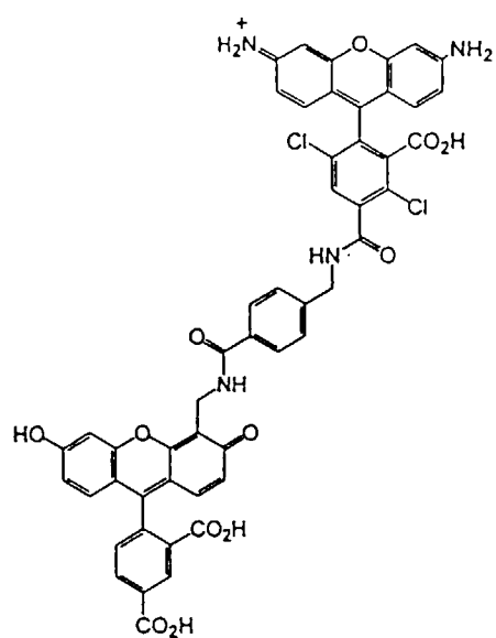
5-CFB-DR110-2
