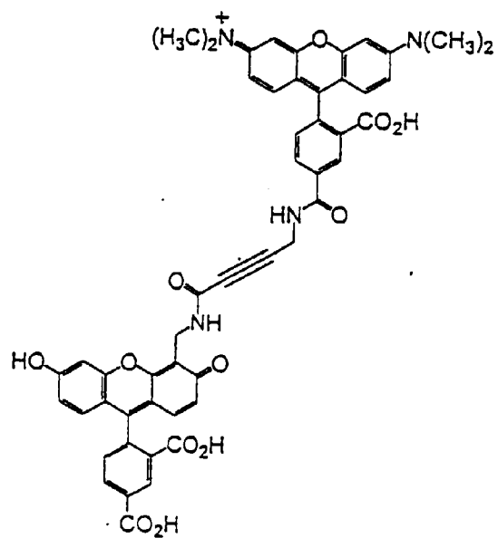
5-TMR-A-CF
