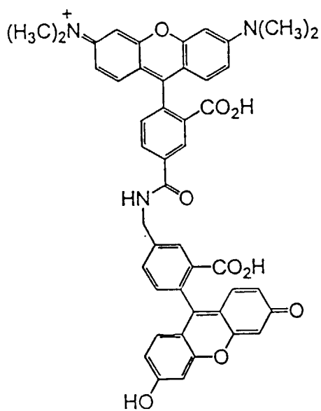
5-TMR-5AMF
