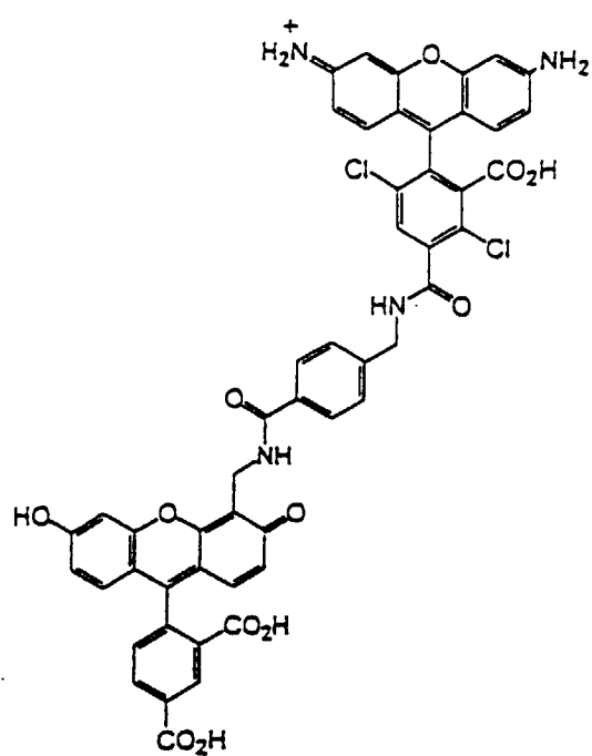
5-CFB-DR110-2
