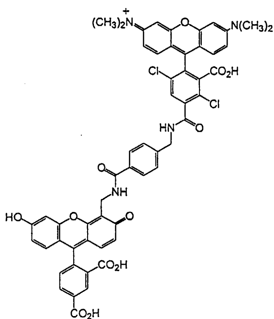
5-CFB-DTMR-2
