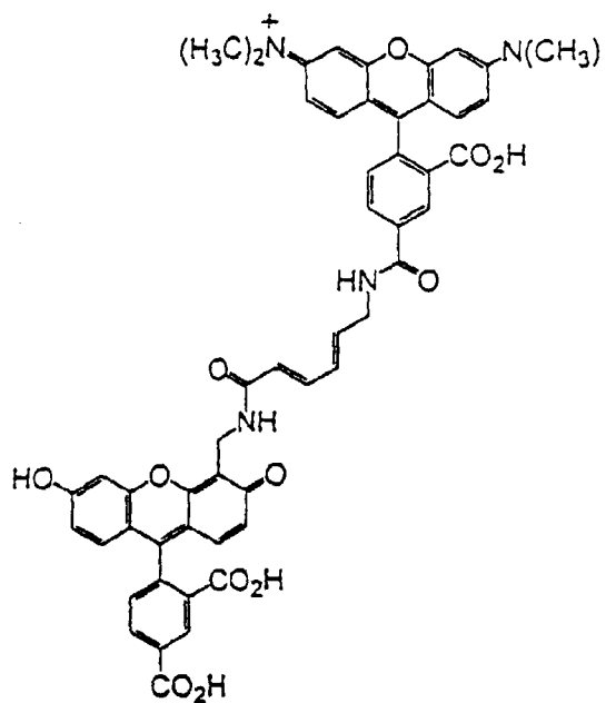
5-TMR-D-CF
