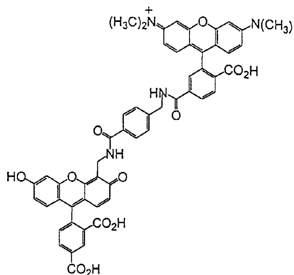
6-TMR-B-CF
