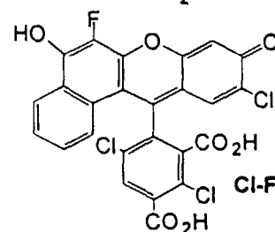
5-carboxy-HEX
