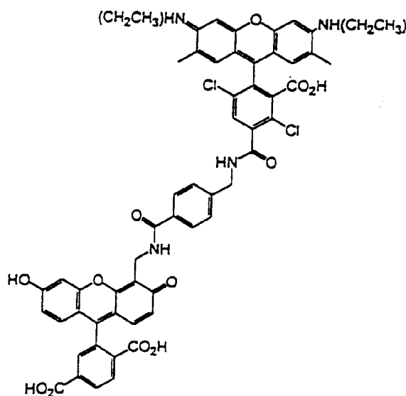
6-CFB-DR6G-2
