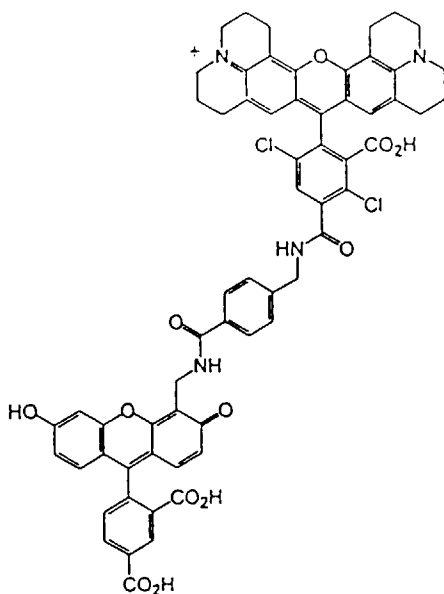
5-CFB-DROX-2
