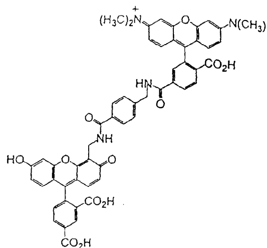
6-TMR-B-CF
