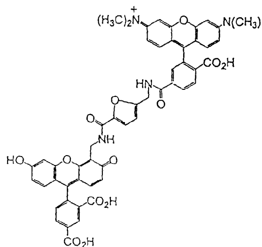
6-TMR-F-CF
