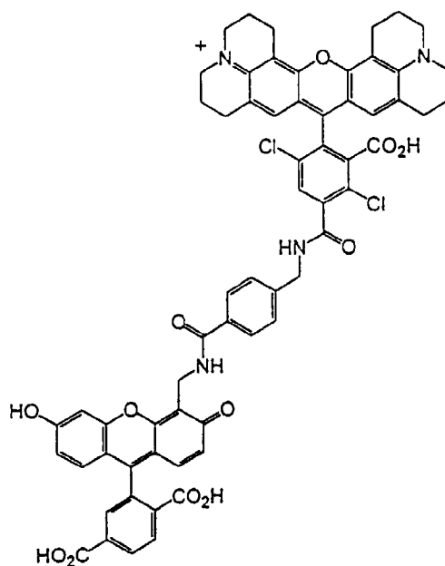
6-CFB-DROX-2
