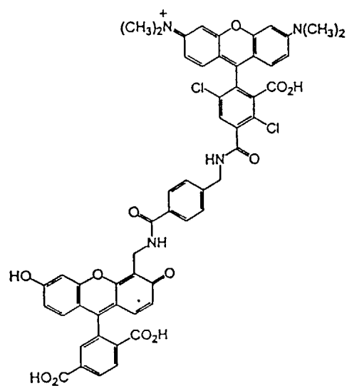
6-CFB-DTMR-2
