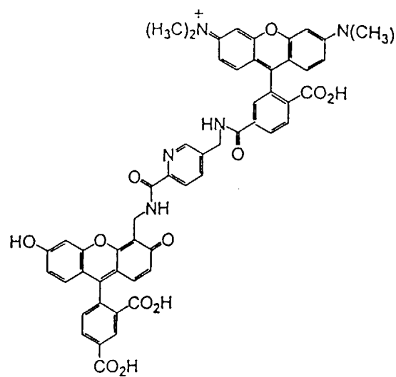
6-TMR-P-CF
