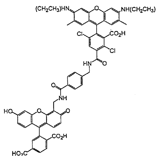
6-CFB-DR6G-2
