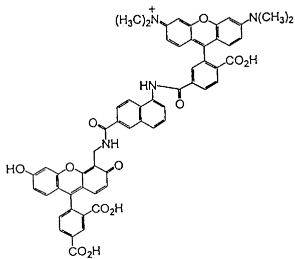
6-TMR-N-CF
