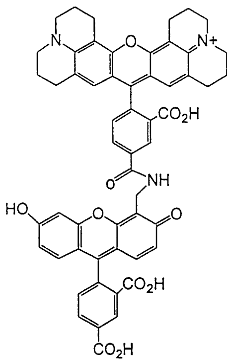
5-ROX-CF
