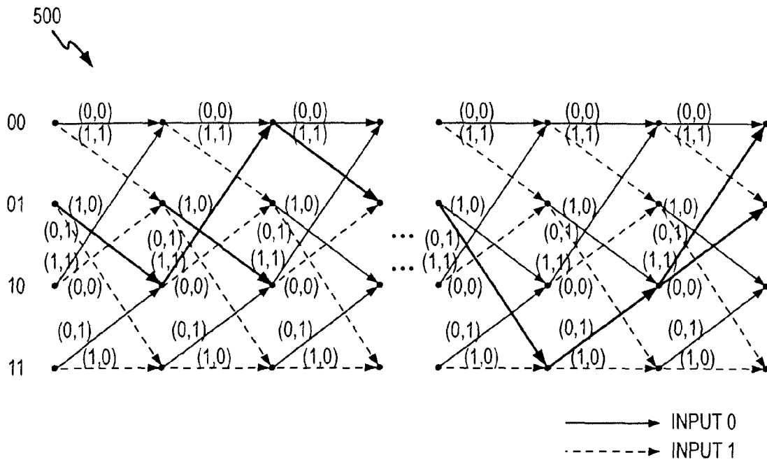
FIG.5 (PRIOR ART)
