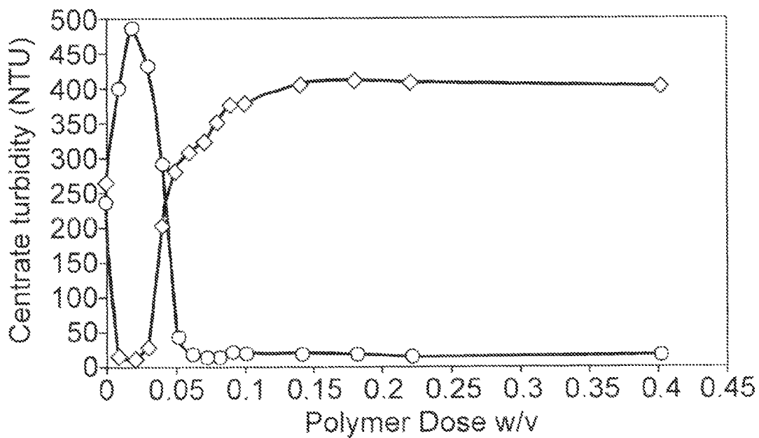
CHO Cell Culture Flocculation, Dosing Effect on Centrate Turbidity; MMW Chitosan vs. Benzyl Modified Polyallylamine with Stimulus
