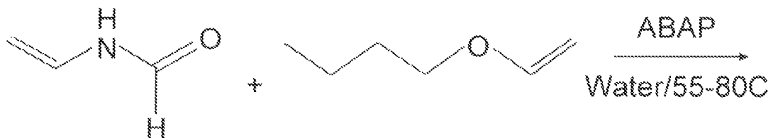
N-vinylformamide
