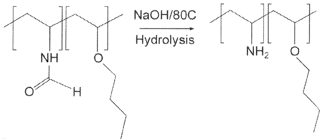
Poly(vinylformamid -co-butylvinylether)
