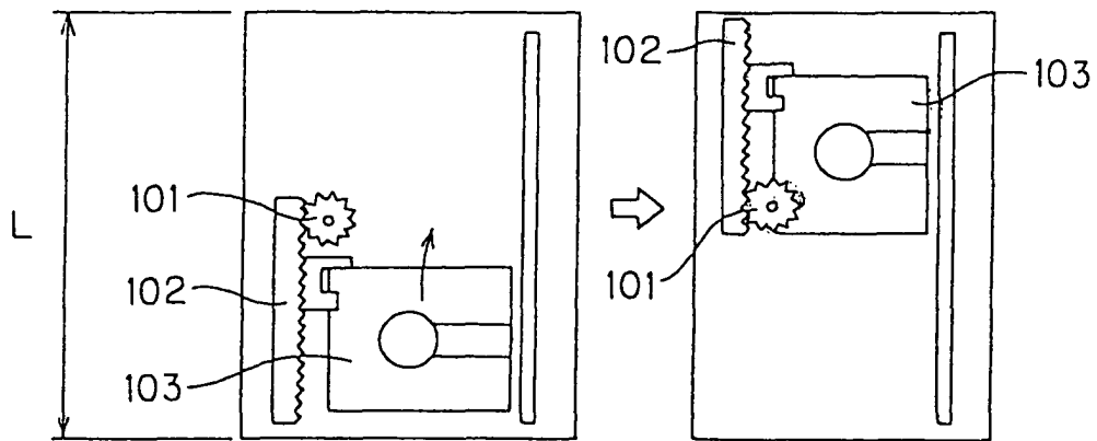
FIG. 15 PRIOR ART
