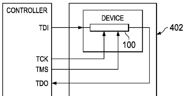
FIG. 4 (PRIOR ART)
