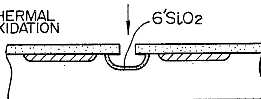
FIG. 8E COATING AND CALCINING
