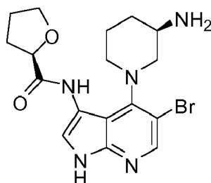
(R)-N-(4-((R)-3-Aminopiperidin-1-yl)-5-bromo-1H-pyrrolo[2,3-b]pyridin-3-yl)tetrahydrofuran-2-carboxamide
