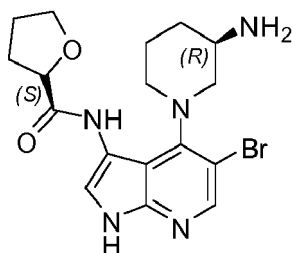
(S)-N-(4-((R)-3-Aminopiperidin-1-yl)-5-bromo-1H-pyrrolo[2,3-b]pyridin-3-yl)tetrahydrofuran-2-carboxamide
