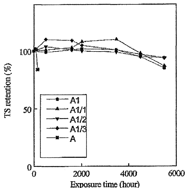
Fig. 1 TS retention (%) for stretched PP (A) films (i.e. A1/I - A1/3) after accelerated weathering by Q-UV.
