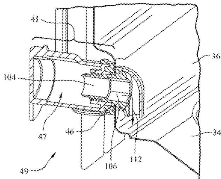
Fig. 7 (PRIOR ART)
