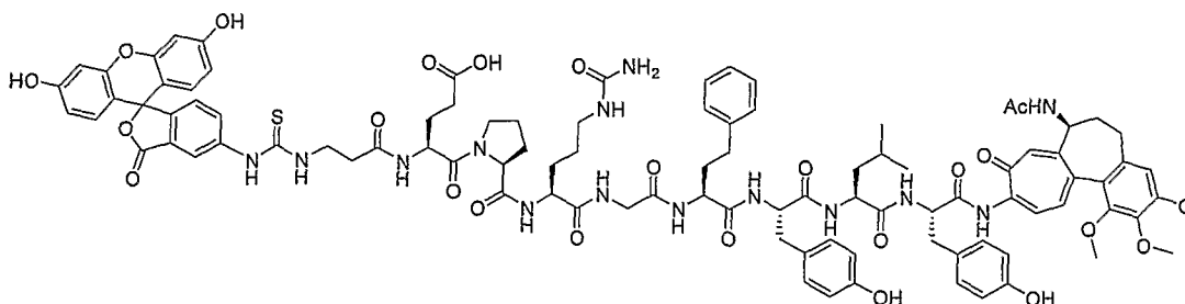
5 fluo-bala-glu-pro-cit-gly-hof-tyr-leu-tyr-colch
