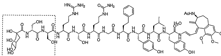
Quinic-D-Ser-D-Ser-Arg-Ser-Cit-Gly-HoPhe-Tyr-Leu-Tyr-Warhead
