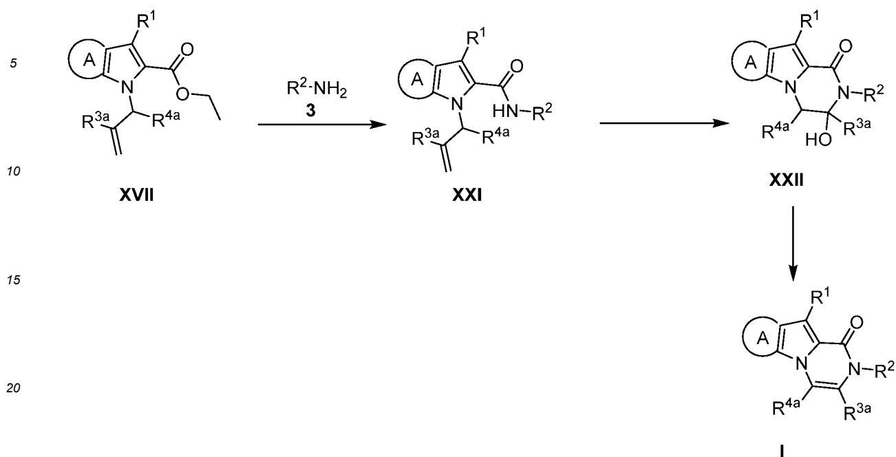
Scheme 8
