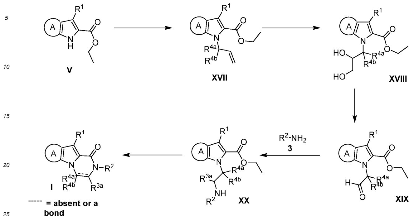
Scheme 7
