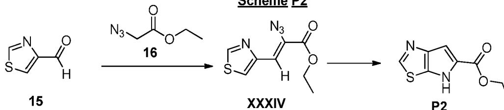
Scheme P2
