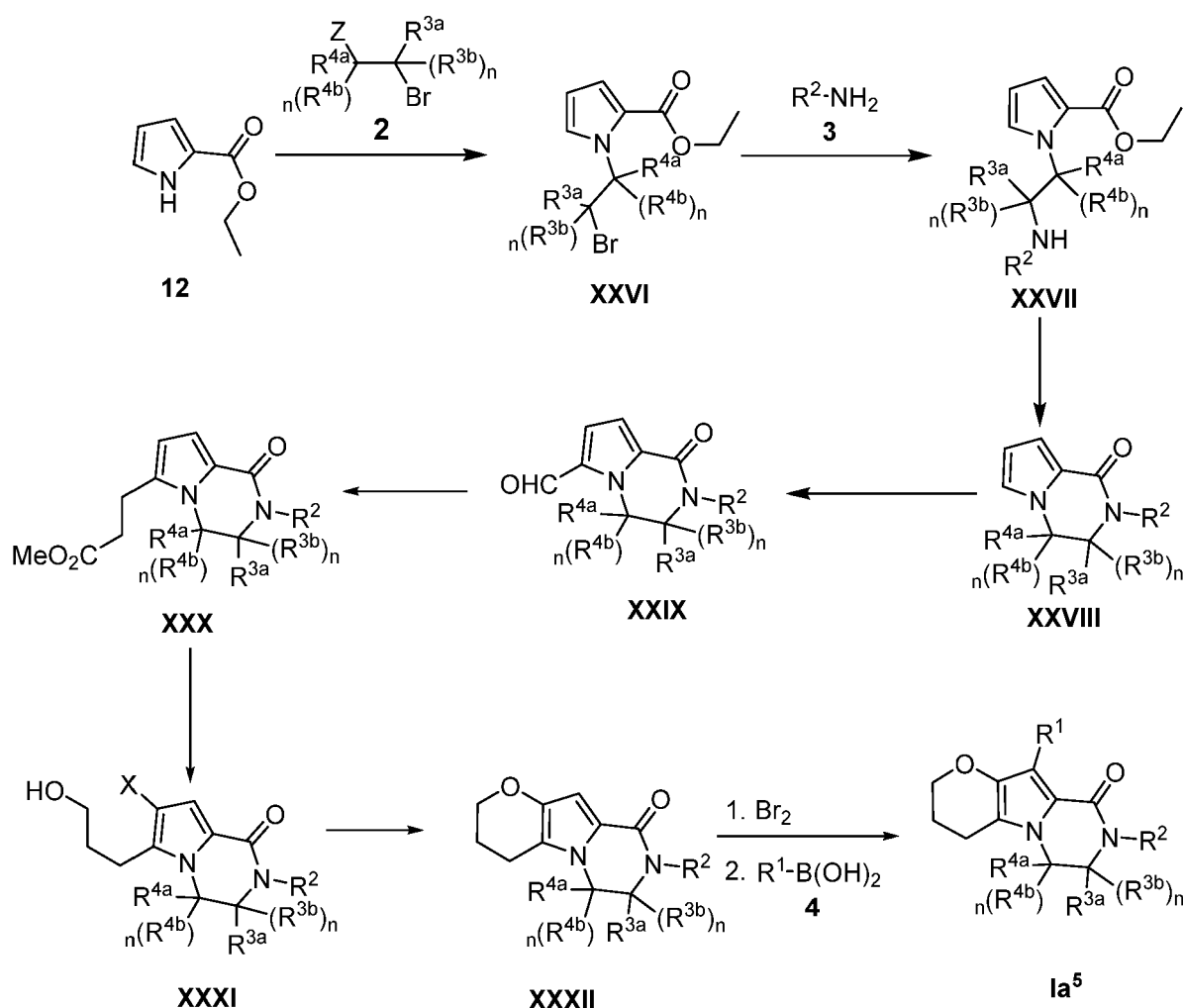
Scheme 11
