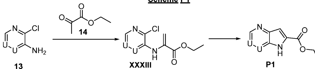
Scheme P1
