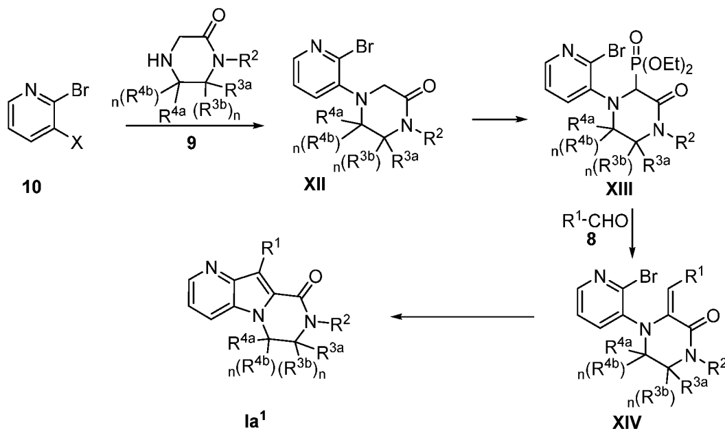
Scheme 5
