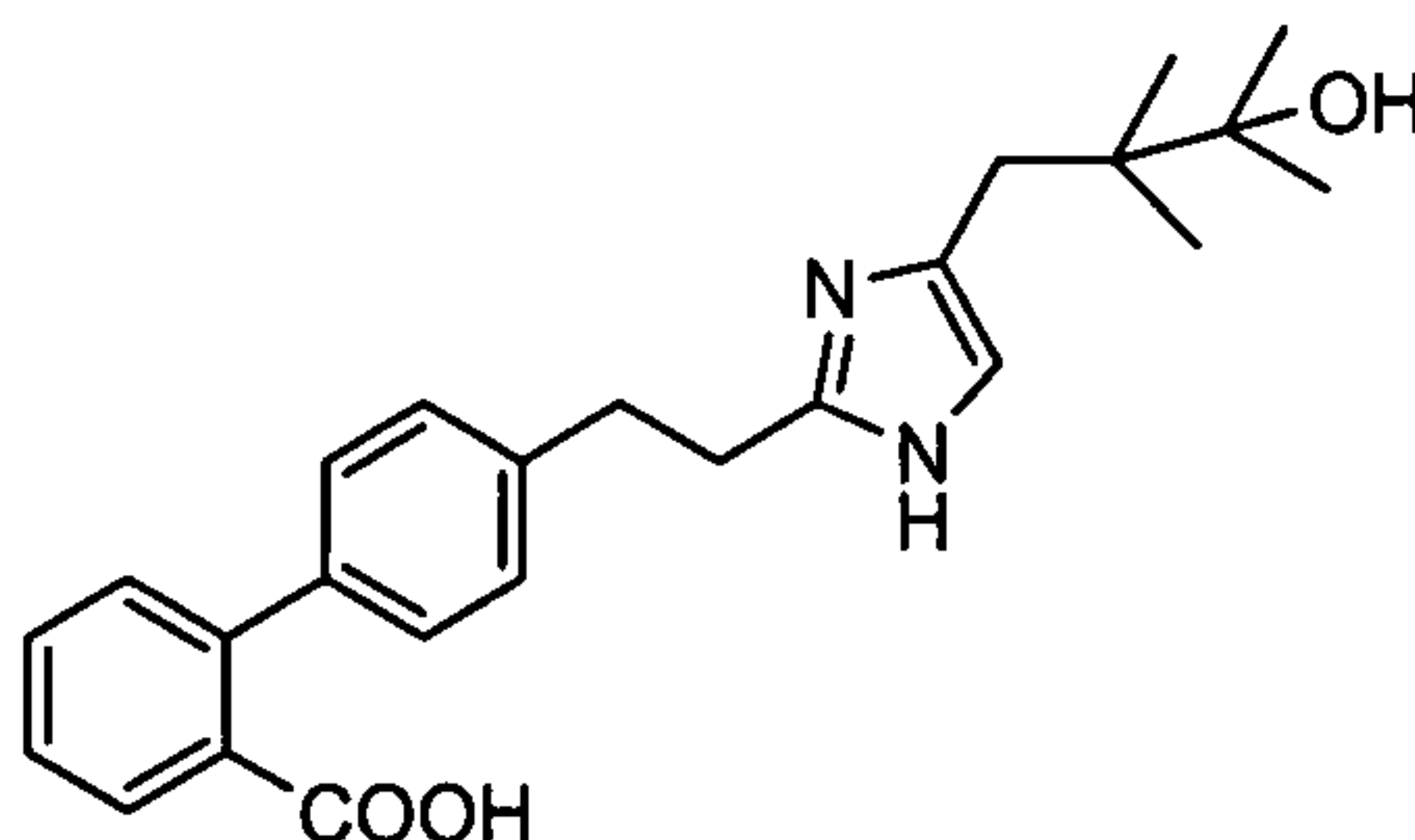
4'-{2-[4-(2,2-Dimethyl-3-hydroxy-3-methylbutyl)-1H-imidazol-2-yl]ethyl}biphenyl-2-carboxylic Acid
