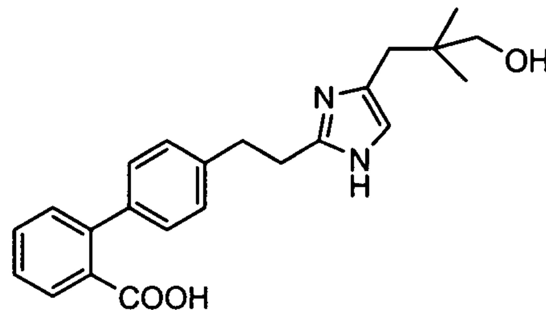
4'-{2-[4-(2,2-Dimethyl-3-hydroxypropyl)-1H-imidazol-2-yl]ethyl}biphenyl-2-carboxylic Acid
