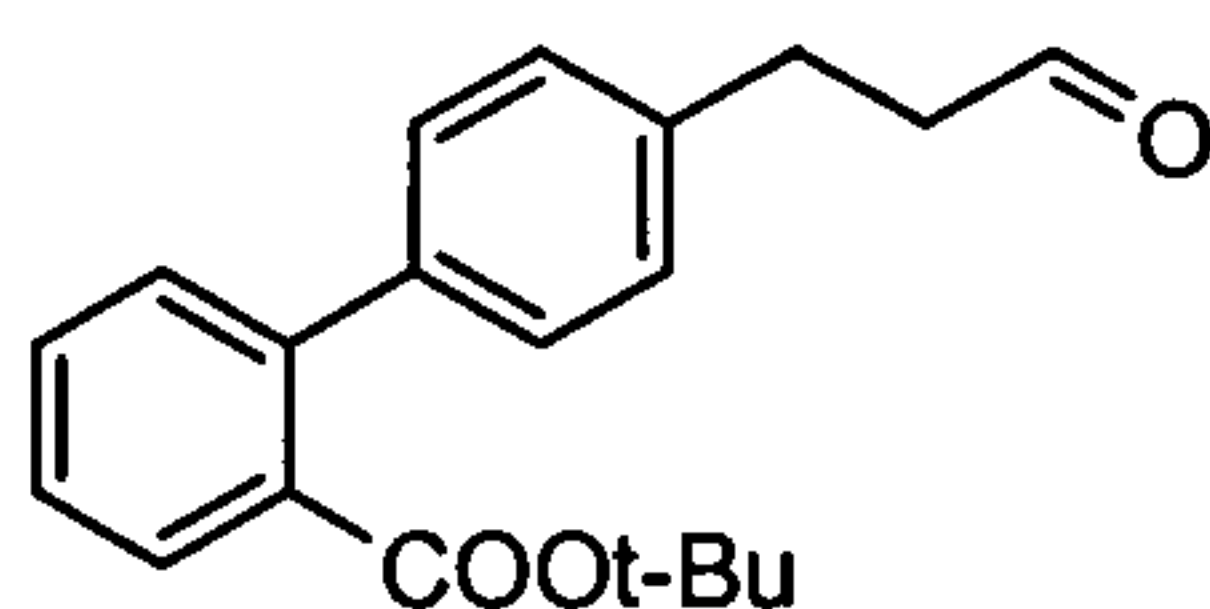
tert-Butyl 4'-(3-oxopropyl)biphenyl-2-carboxylate
