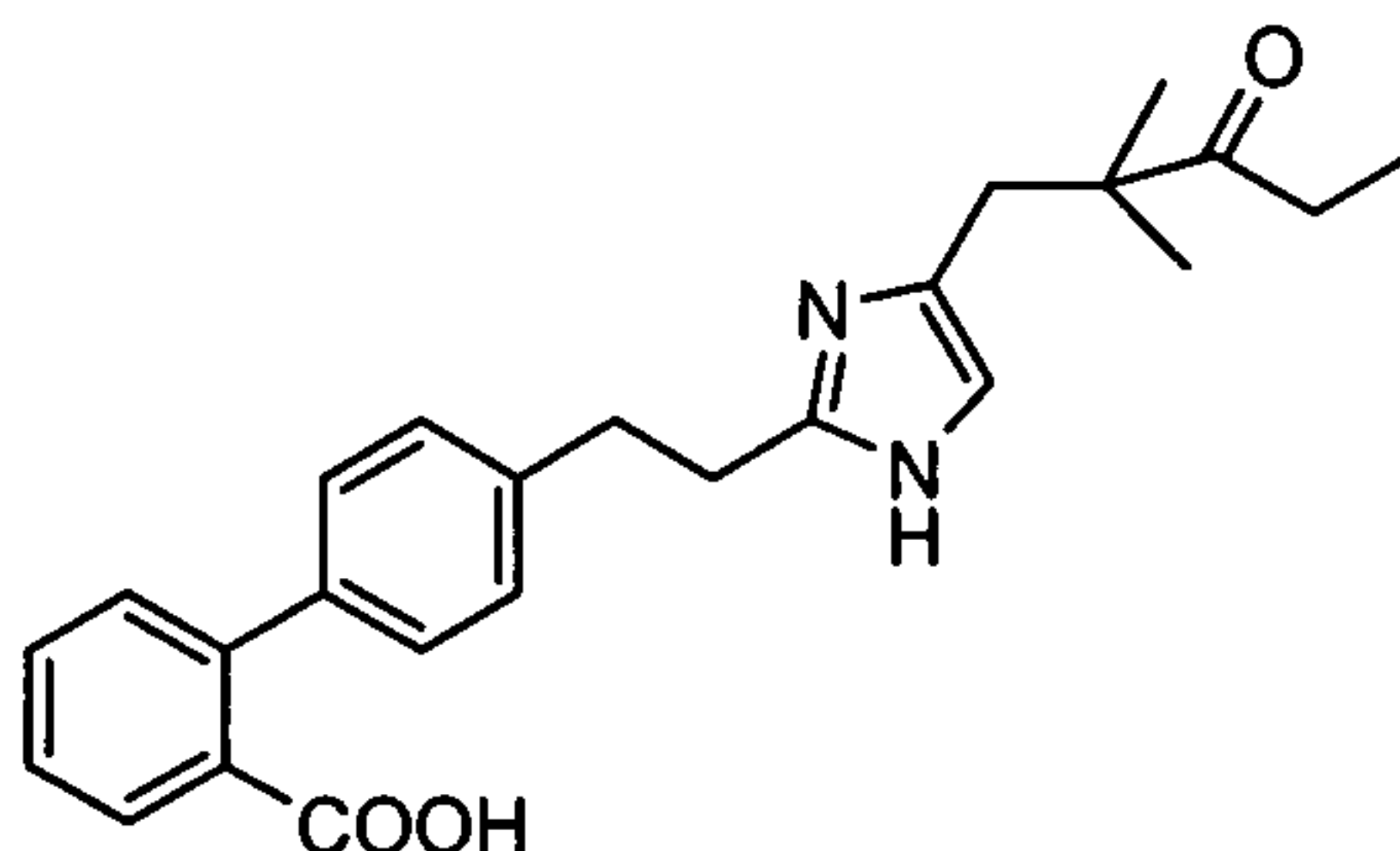
4'-{2-[4-(2,2-Dimethyl-3-oxopentyl)-1H-imidazol-2-yl]ethyl}biphenyl-2-carboxylic Acid
