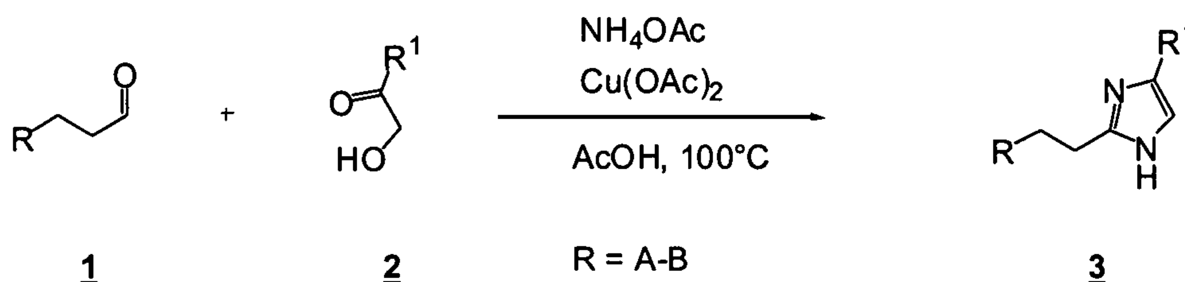
Scheme 1
