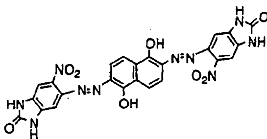
Comparative dye a
