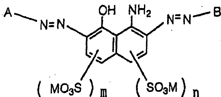
General formula (III)
