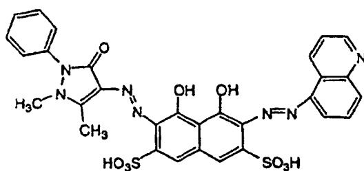
Comparative dye d
