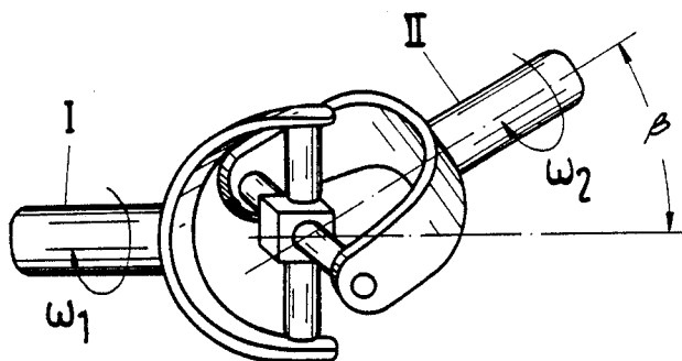
Fig. 8 (PRIOR ART)
