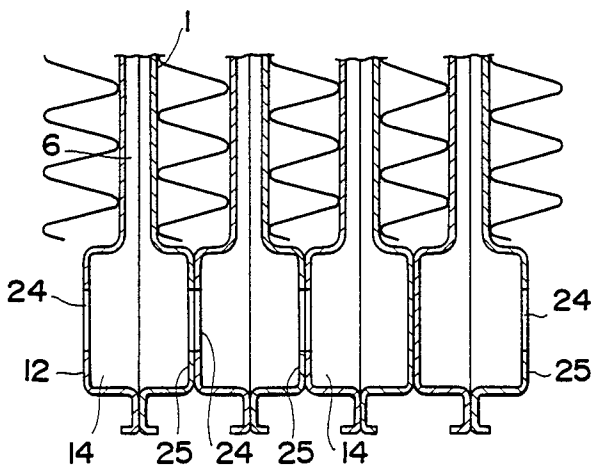
FIG. 10 PRIOR ART
