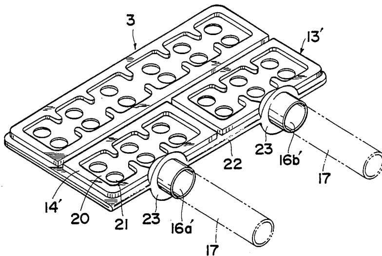
FIG. 9 PRIOR ART
