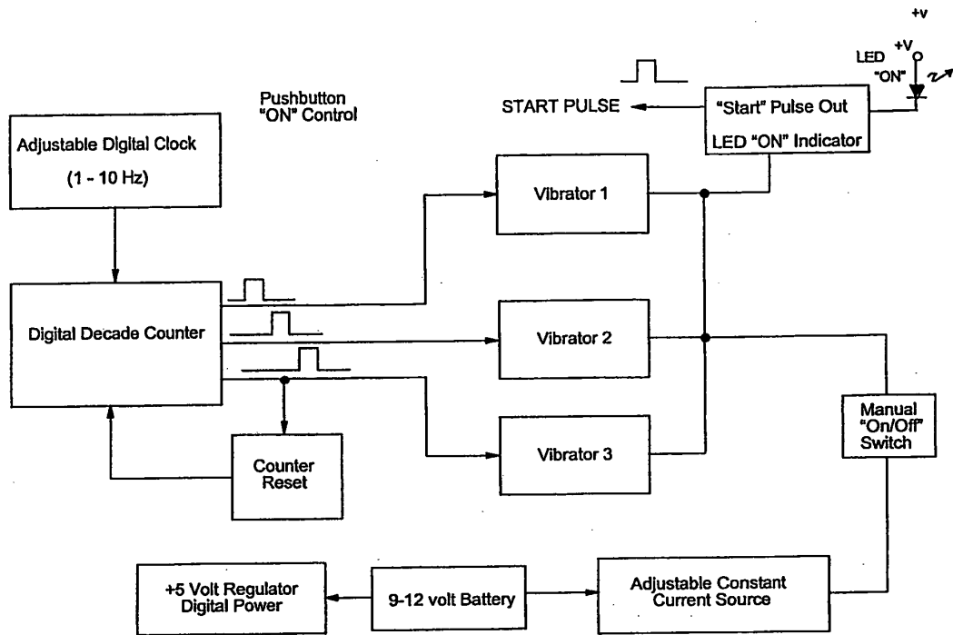
BLOCK DIAGRAM VIBRO-TACTILE STIMULATOR NTM 6/27/2006
