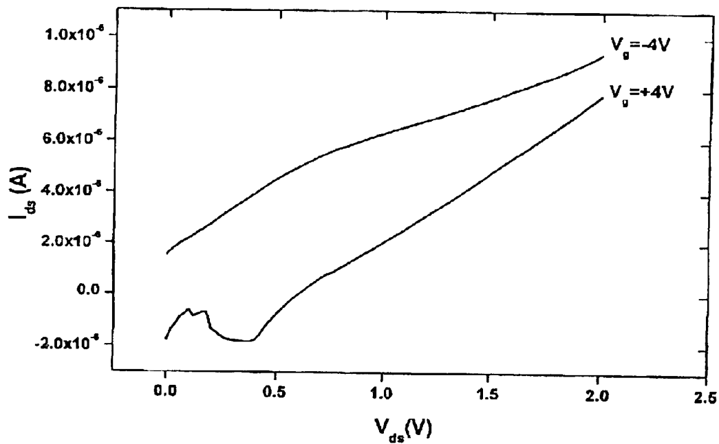
FIGURE 6B
