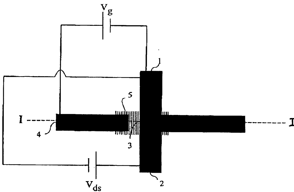
FIGURE 1C
