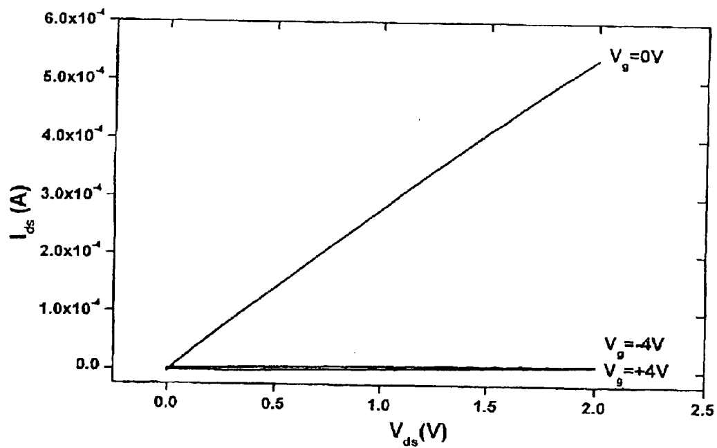
FIGURE 6A
