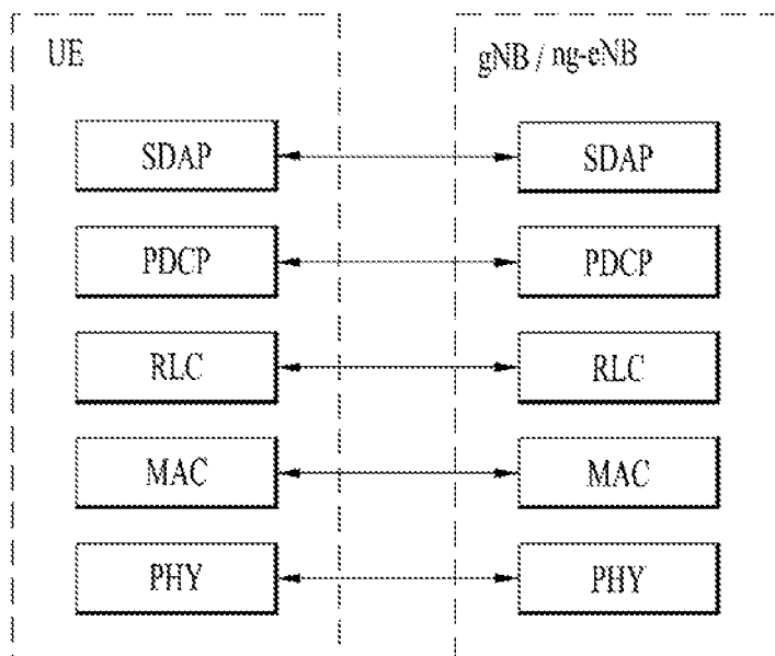
(b) User-Plane Protocol Stack
