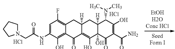
Scheme 5. 1.83-kg batch
