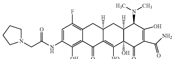
Epimer (TP-498)
