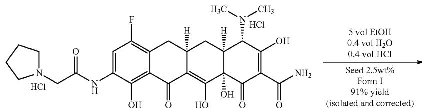
Scheme 3. 300-g scale up of Form I Process
