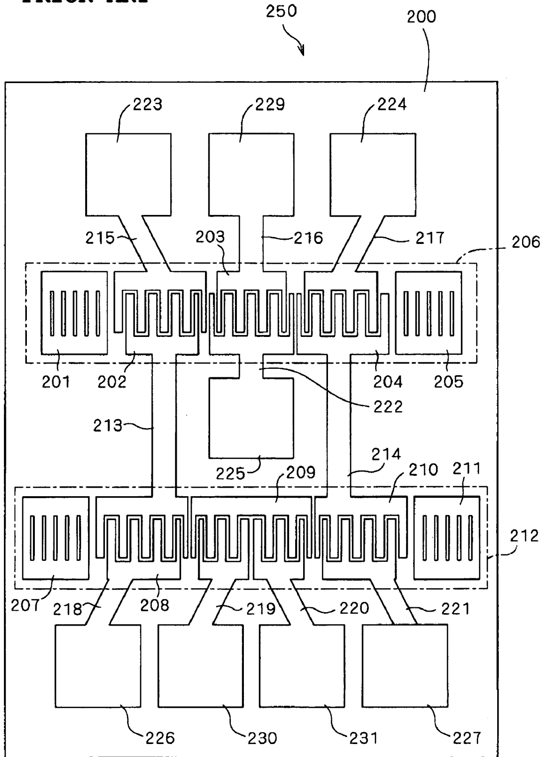
FIG. 2 PRIOR ART
