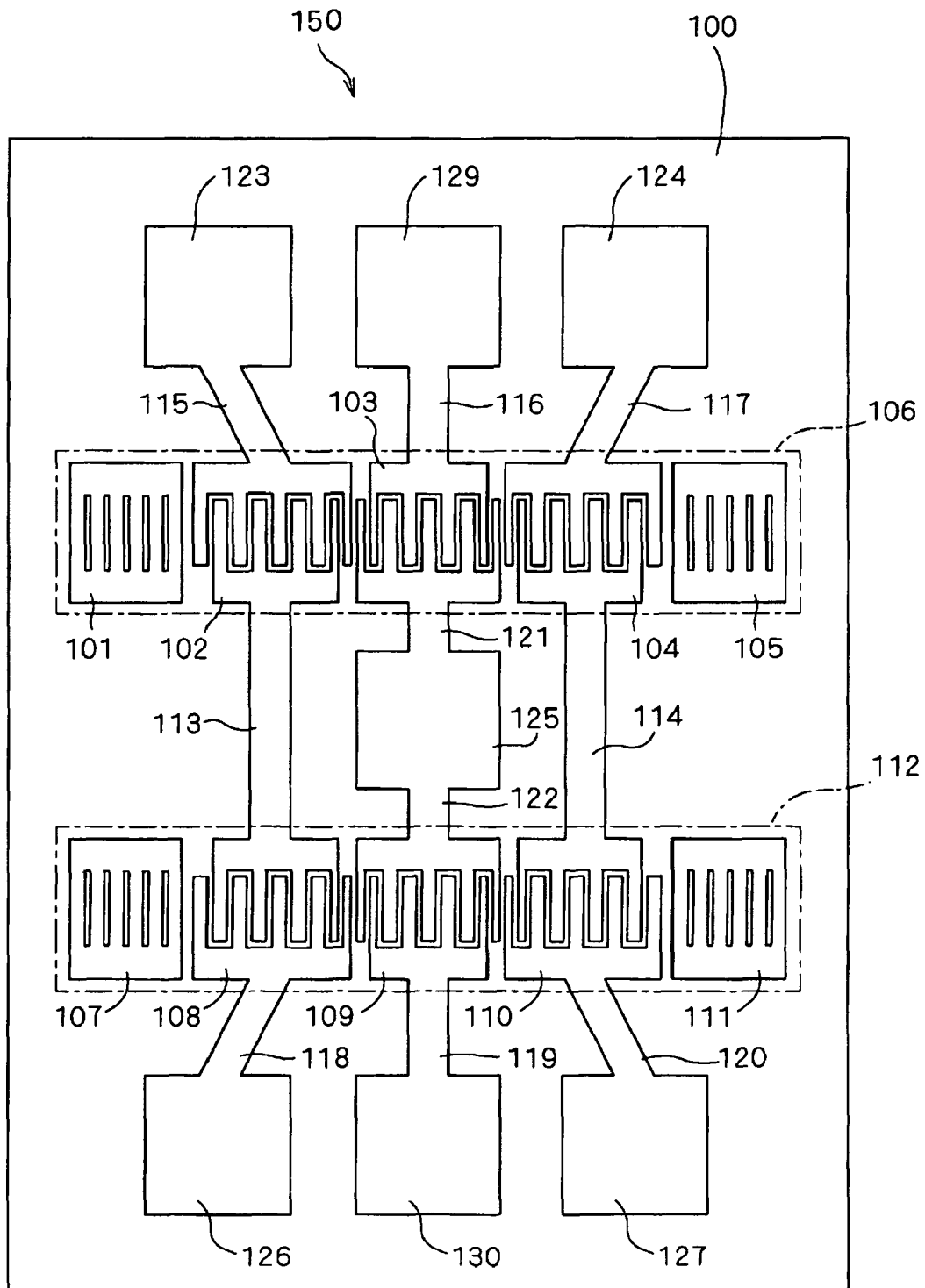
FIG. 1 PRIOR ART
