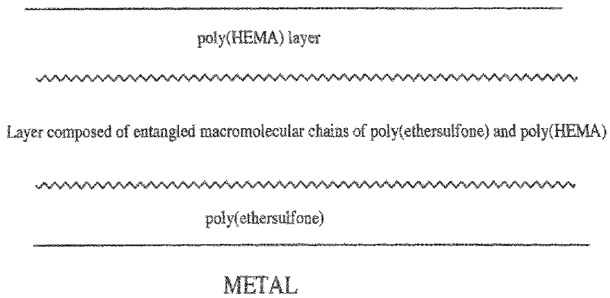
Figure 3. Schematic representation of the entanglement layer which is responsible for the apparent adhesion of poly(HEMA) to the stent surface.
