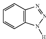
BtH Benzotriazole
