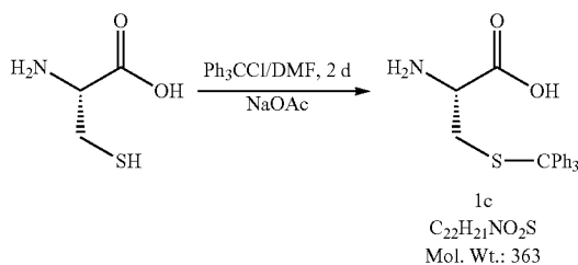
2-Amino-3-tritylsulfanyl-propionic acid (S-Trityl-L-cysteine) (1c)
