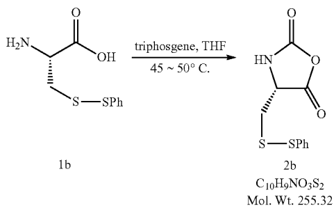
(R)-4-((phenyldisulfanyl)methyl)oxazolidine-2,5-dione (2b)
