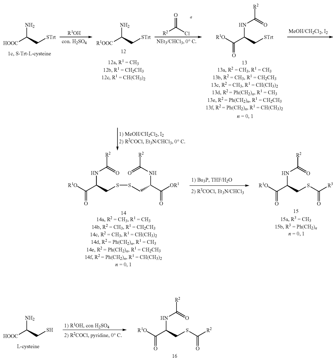
Synthesis of Protected Analogs with Various Groups to Alter the Partition Coefficients Scheme 4
