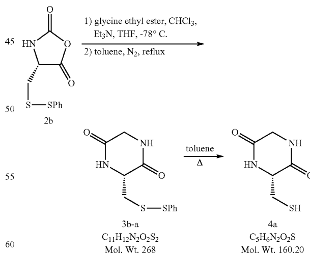
2,5-piperazinedione, 3-(mercaptomethyl)-(4a)
