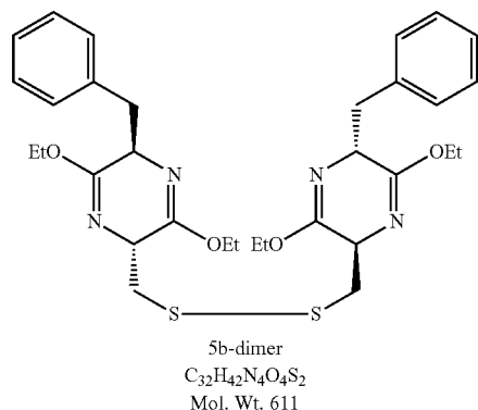
1,2-Bis(((2R,5R)-5-benzyl-3,6-diethoxy-2,5-dihydro-pyrazin-2-yl)methyl)disulfane (5b-dimer)
