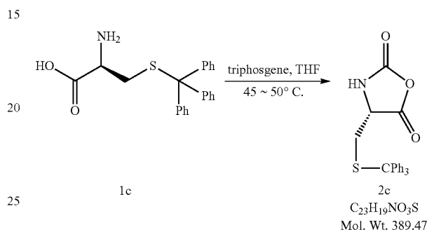
4-Tritylsulfanylmethyl-oxazolidine-2,5-dione (2c)
