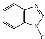
BtCl 1-Chlorobenzotriazole
