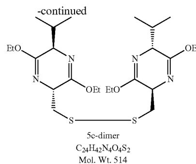
1,2-Bis(((2R,5R)-3,6-diethoxy-5-isopropyl-2,5-dihydro-pyrazin-2-yl)methyl)disulfane (5c-dimer)
