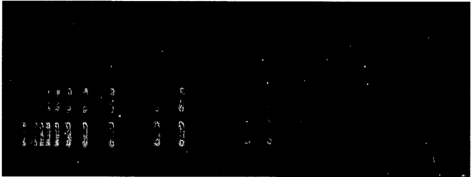
FIG. 11 Post-DNA Gel Staining with Dye No. 29 of Table 1
