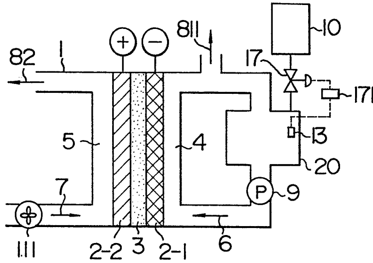
FIG. 4 PRIOR ART
