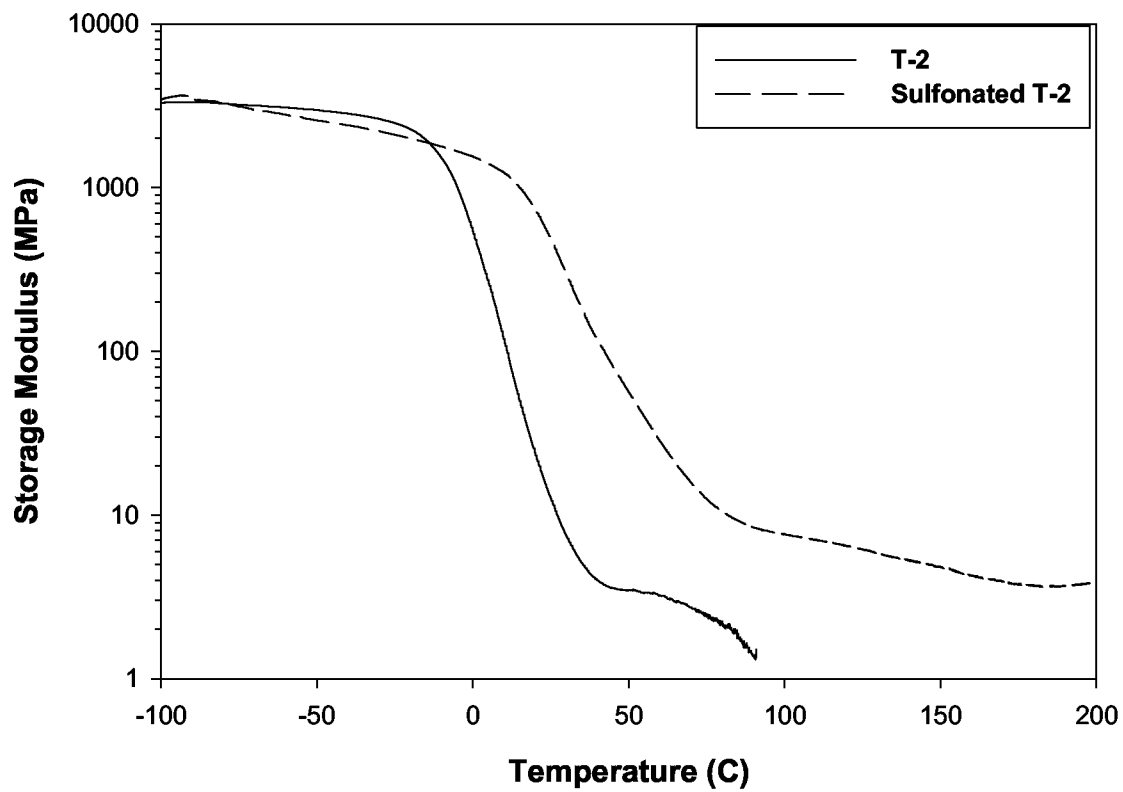
Figure 2 Polymer T-2 Before and After Sulfonation
