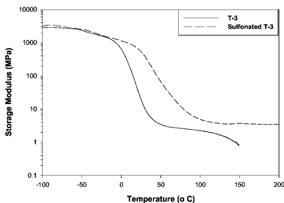
Polymer T-3 Before and After Sulfonation
