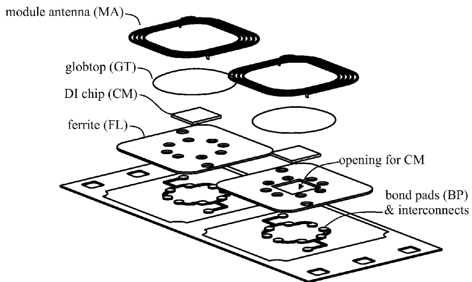
FIG.6C DIF Module with Ferrite Layer
