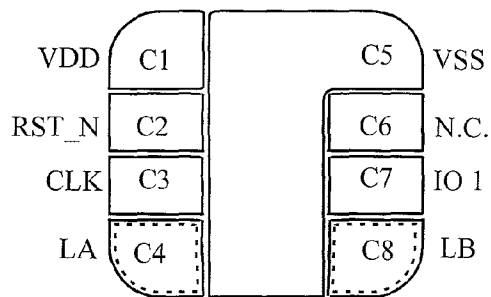
Contact Pad Layout/Assignments
