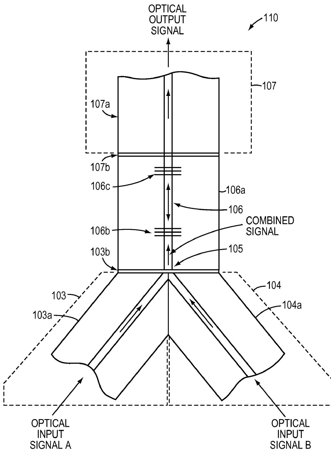
ALL-OPTICAL LOGICAL GATE IMPLEMENTED WITH OPTICAL FIBERS
