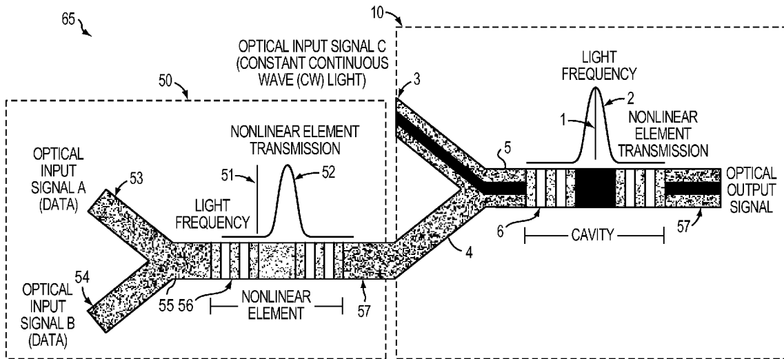
ALL-OPTICAL XNOR GATE WITH LOGIC LEVEL RESTORATION
