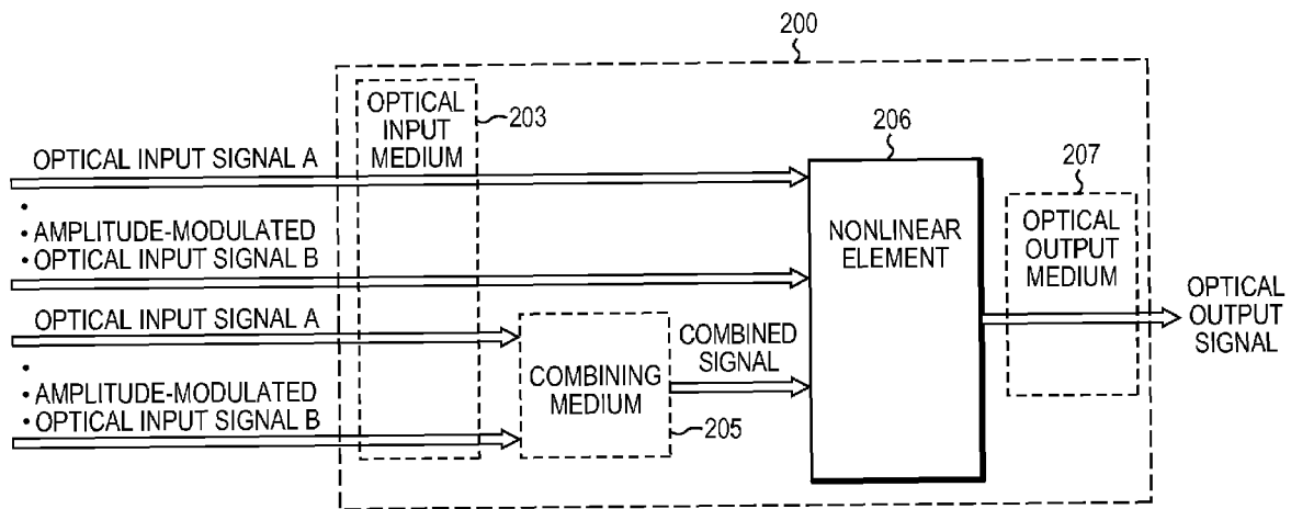
GENERALIZED ALL-OPTICAL LOGICAL GATE
